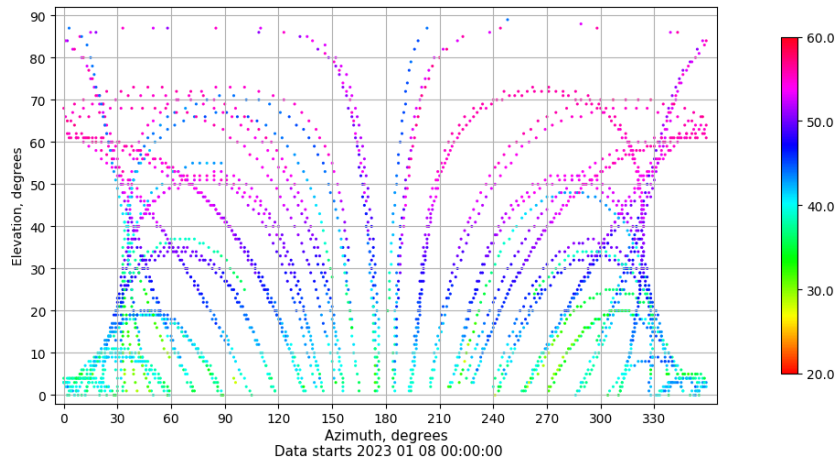
Azimuth-elevation plot for station XIXO. Signal to Noise S1C Data file XIXO00ESP_R_2023008.xtr
