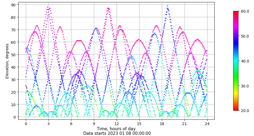
Time-elevation plot for station XIXO. Signal to Noise S1C Data file XIXO00ESP_R_2023008.xtr
