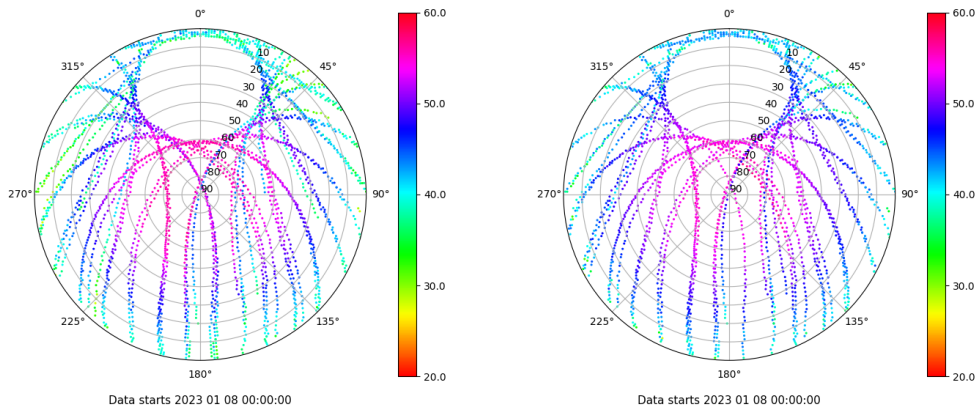
Skyplot for station XIXO. Signal to Noise S1C Data file XIXO00ESP_R_2023008.xtr Skyplot for station XIXO. Signal to Noise S2C Data file XIXO00ESP_R_2023008.xtr
