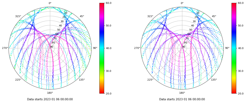
Skyplot for station XIXO. Signal to Noise S1C Data file XIXO00ESP_R_2023006.xtr Skyplot for station XIXO. Signal to Noise S2C Data file XIXO00ESP_R_2023006.xtr
