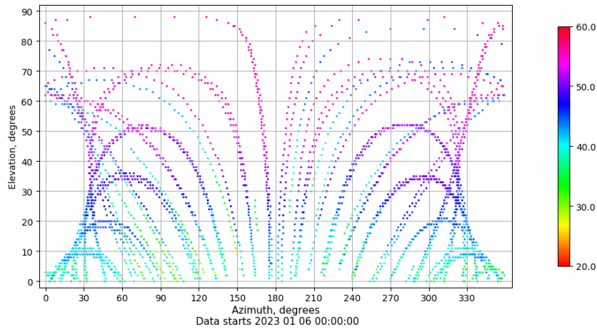
Azimuth-elevation plot for station XIXO. Signal to Noise S1C Data file XIXO00ESP_R_2023006.xtr
