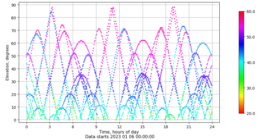
Time-elevation plot for station XIXO. Signal to Noise S1C Data file XIXO00ESP_R_2023006.xtr
