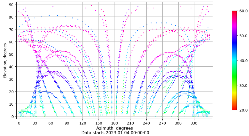
Azimuth-elevation plot for station XIXO. Signal to Noise S1C Data file XIXO00ESP_R_2023004.xtr
