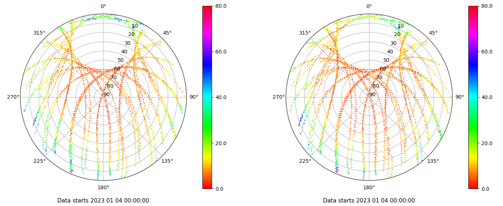
Skyplot for station XIXO. Parameter M1C Data file XIXO00ESP_R_2023004.xtr Skyplot for station XIXO. Parameter M2C Data file XIXO00ESP_R_2023004.xtr
