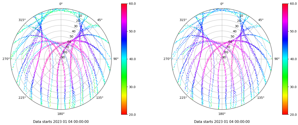
Skyplot for station XIXO. Signal to Noise S1C Data file XIXO00ESP_R_2023004.xtr Skyplot for station XIXO. Signal to Noise S2C Data file XIXO00ESP_R_2023004.xtr
