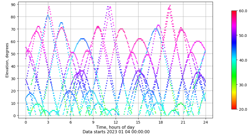
Time-elevation plot for station XIXO. Signal to Noise S1C Data file XIXO00ESP_R_2023004.xtr
