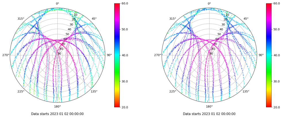
Skyplot for station XIXO. Signal to Noise S1C Data file XIXO00ESP_R_2023002.xtr Skyplot for station XIXO. Signal to Noise S2C Data file XIXO00ESP_R_2023002.xtr
