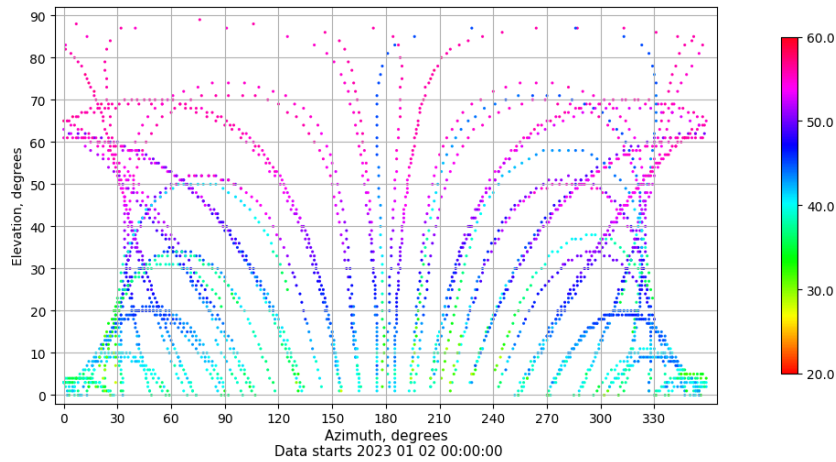
Azimuth-elevation plot for station XIXO. Signal to Noise S1C Data file XIXO00ESP_R_2023002.xtr
