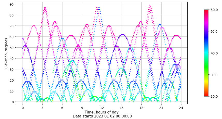
Time-elevation plot for station XIXO. Signal to Noise S1C Data file XIXO00ESP_R_2023002.xtr
