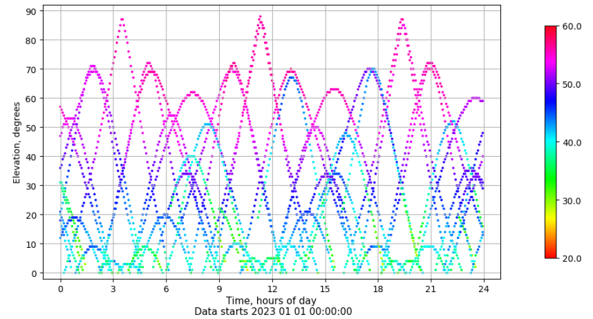
Time-elevation plot for station XIXO. Signal to Noise S1C Data file XIXO00ESP_R_2023001.xtr
