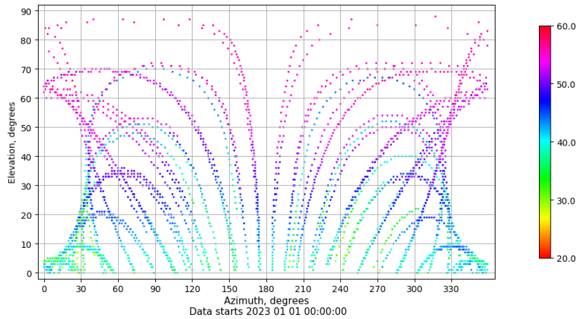
Azimuth-elevation plot for station XIXO. Signal to Noise S1C Data file XIXO00ESP_R_2023001.xtr
