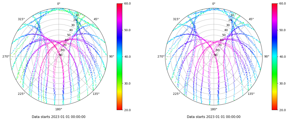
Skyplot for station XIXO. Signal to Noise S1C Data file XIXO00ESP_R_2023001.xtr Skyplot for station XIXO. Signal to Noise S2C Data file XIXO00ESP_R_2023001.xtr
