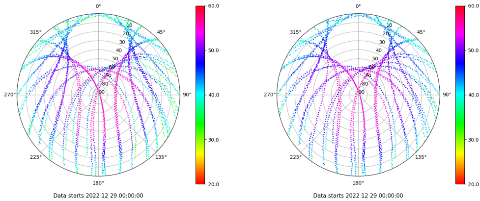
Skyplot for station XIXO. Signal to Noise S1C Data file XIXO00ESP_R_2022363.xtr Skyplot for station XIXO. Signal to Noise S2C Data file XIXO00ESP_R_2022363.xtr
