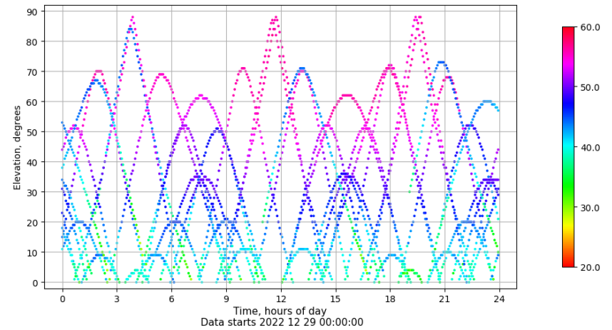
Time-elevation plot for station XIXO. Signal to Noise S1C Data file XIXO00ESP_R_2022363.xtr
