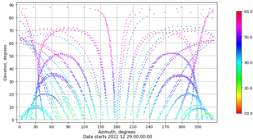
Azimuth-elevation plot for station XIXO. Signal to Noise S1C Data file XIXO00ESP_R_2022363.xtr
