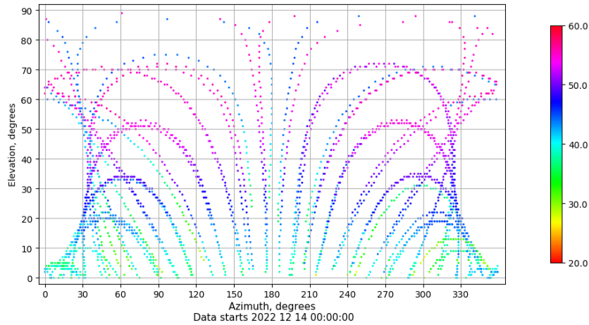
Azimuth-elevation plot for station XIXO. Signal to Noise S1C Data file XIXO00ESP_R_2022348.xtr
