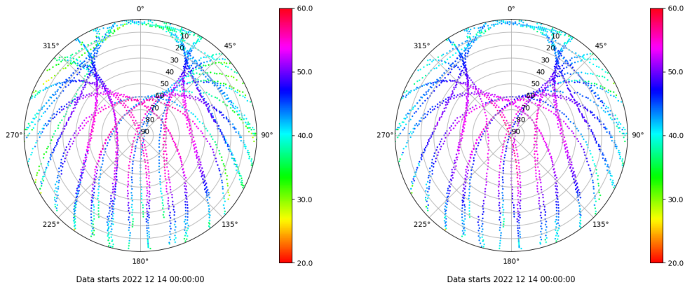
Skyplot for station XIXO. Signal to Noise S1C Data file XIXO00ESP_R_2022348.xtr Skyplot for station XIXO. Signal to Noise S2C Data file XIXO00ESP_R_2022348.xtr
