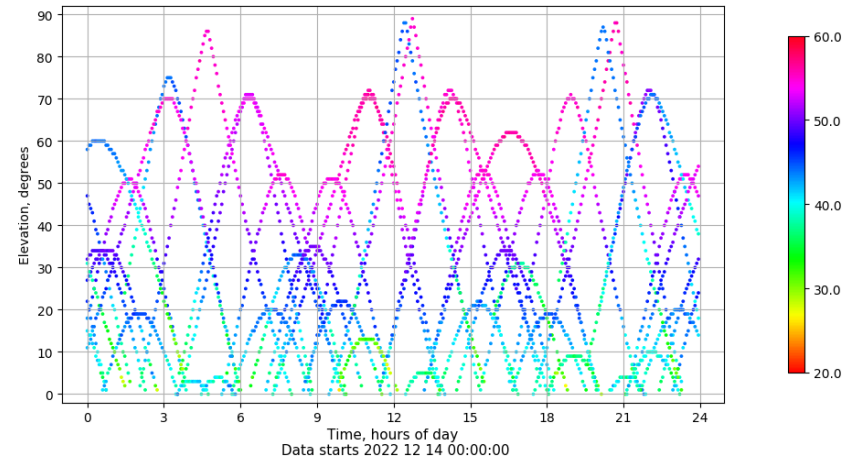
Time-elevation plot for station XIXO. Signal to Noise S1C Data file XIXO00ESP_R_2022348.xtr
