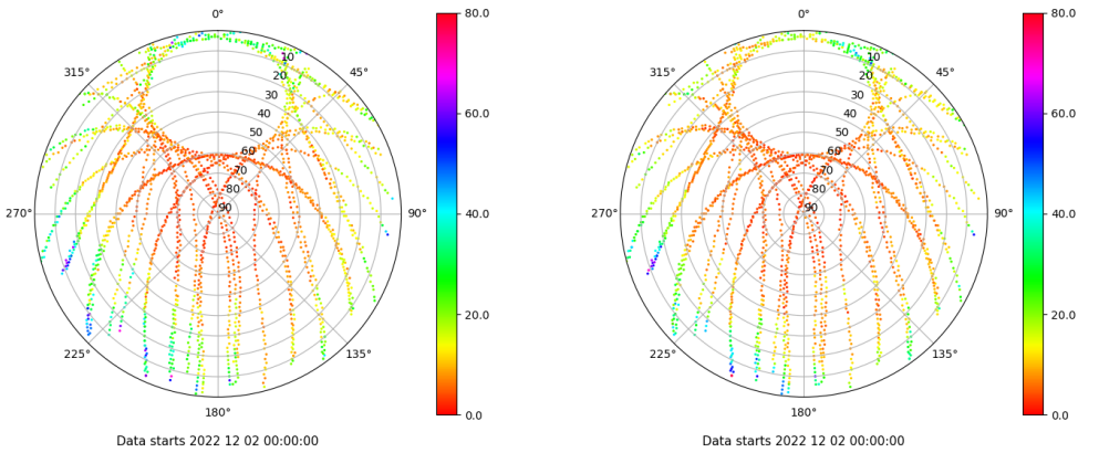
Skyplot for station XIXO. Parameter M1C Data file XIXO00ESP_R_2022336.xtr Skyplot for station XIXO. Parameter M2C Data file XIXO00ESP_R_2022336.xtr
