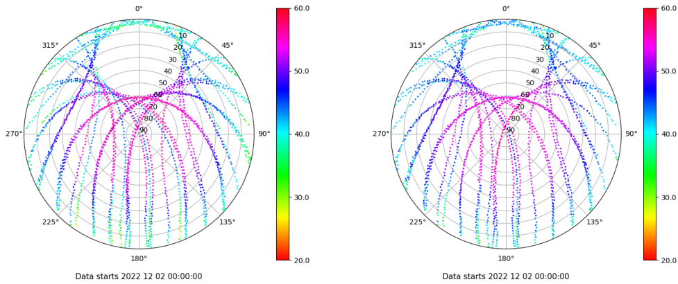
Skyplot for station XIXO. Signal to Noise S1C Data file XIXO00ESP_R_2022336.xtr Skyplot for station XIXO. Signal to Noise S2C Data file XIXO00ESP_R_2022336.xtr
