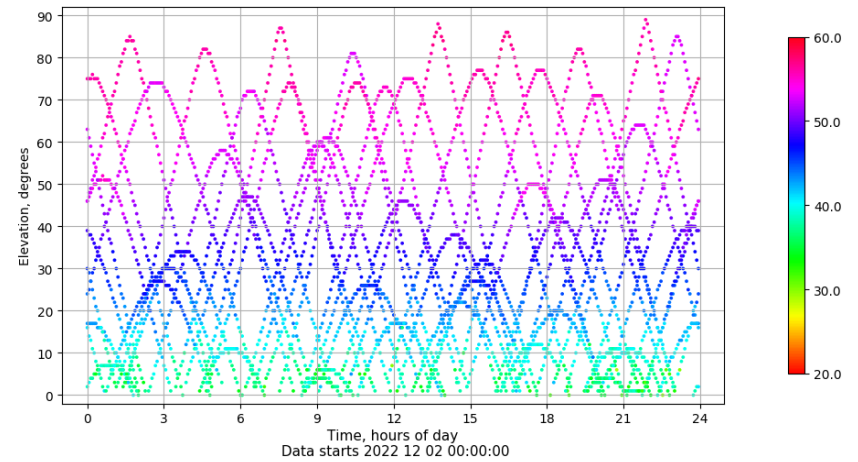
Time-elevation plot for station XIXO. Signal to Noise S1C Data file XIXO00ESP_R_2022336.xtr
