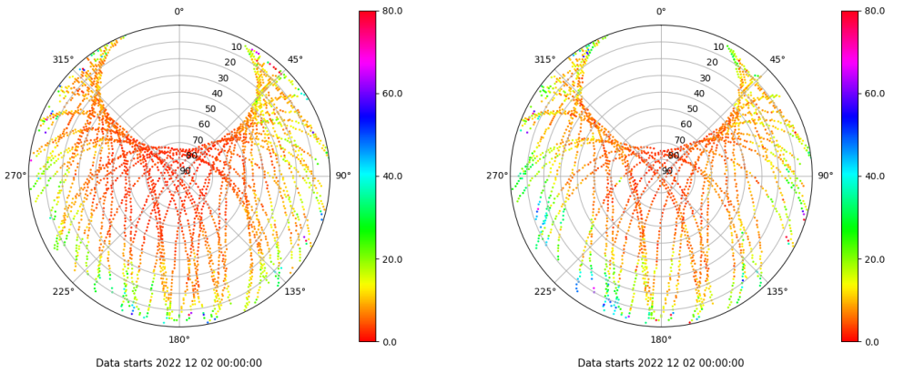
Skyplot for station XIXO. Parameter M1C Data file XIXO00ESP_R_2022336.xtr Skyplot for station XIXO. Parameter M2S Data file XIXO00ESP_R_2022336.xtr
