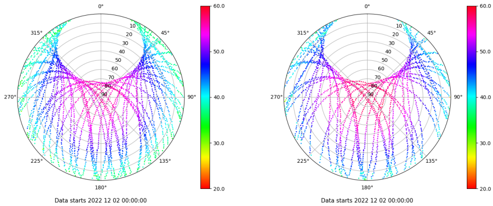
Skyplot for station XIXO. Signal to Noise S1C Data file XIXO00ESP_R_2022336.xtr Skyplot for station XIXO. Signal to Noise S2S Data file XIXO00ESP_R_2022336.xtr
