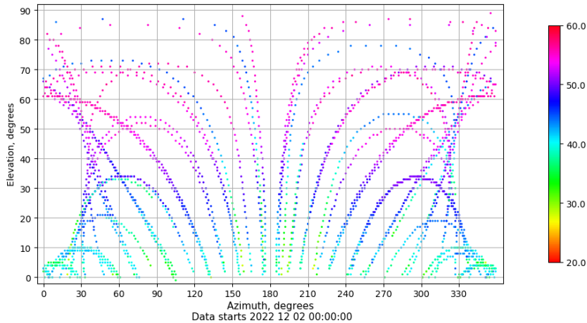
Azimuth-elevation plot for station XIXO. Signal to Noise S1C Data file XIXO00ESP_R_2022336.xtr
