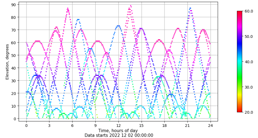
Time-elevation plot for station XIXO. Signal to Noise S1C Data file XIXO00ESP_R_2022336.xtr
