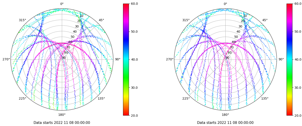
Skyplot for station XIXO. Signal to Noise S1C Data file XIXO00ESP_R_2022312.xtr Skyplot for station XIXO. Signal to Noise S2C Data file XIXO00ESP_R_2022312.xtr
