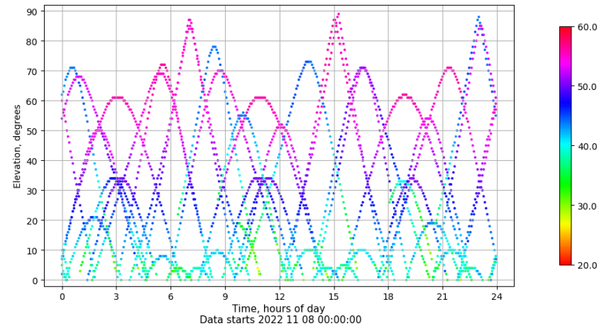
Time-elevation plot for station XIXO. Signal to Noise S1C Data file XIXO00ESP_R_2022312.xtr
