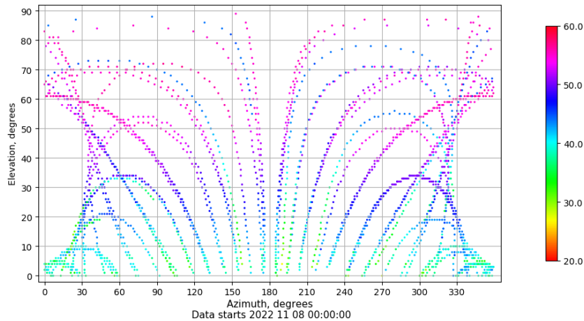
Azimuth-elevation plot for station XIXO. Signal to Noise S1C Data file XIXO00ESP_R_2022312.xtr
