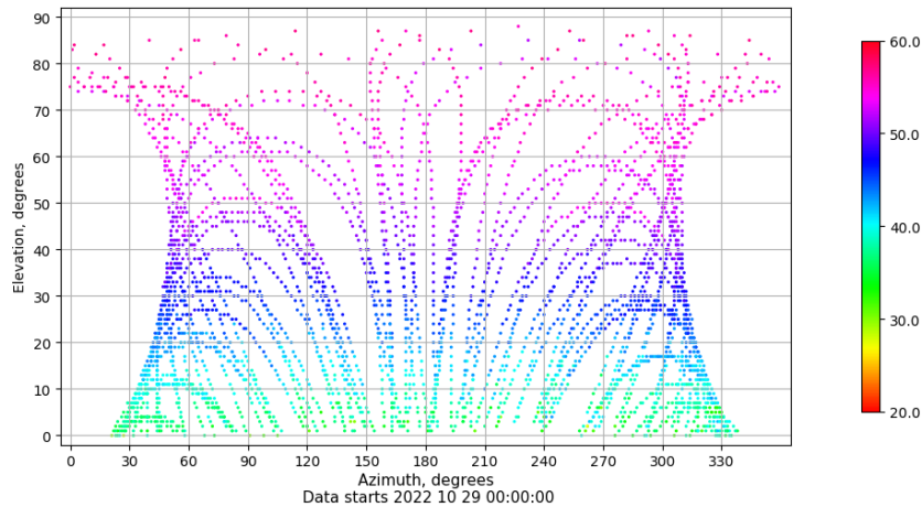
Azimuth-elevation plot for station XIXO. Signal to Noise S1C Data file XIXO00ESP_R_2022302.xtr
