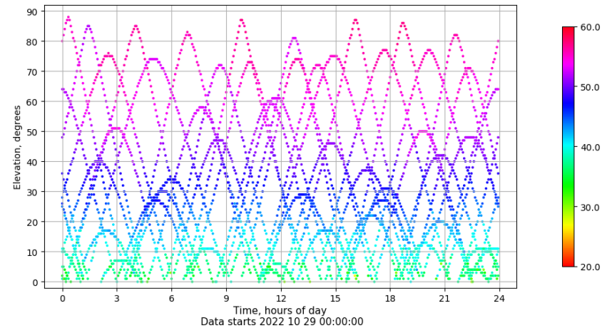
Time-elevation plot for station XIXO. Signal to Noise S1C Data file XIXO00ESP_R_2022302.xtr
