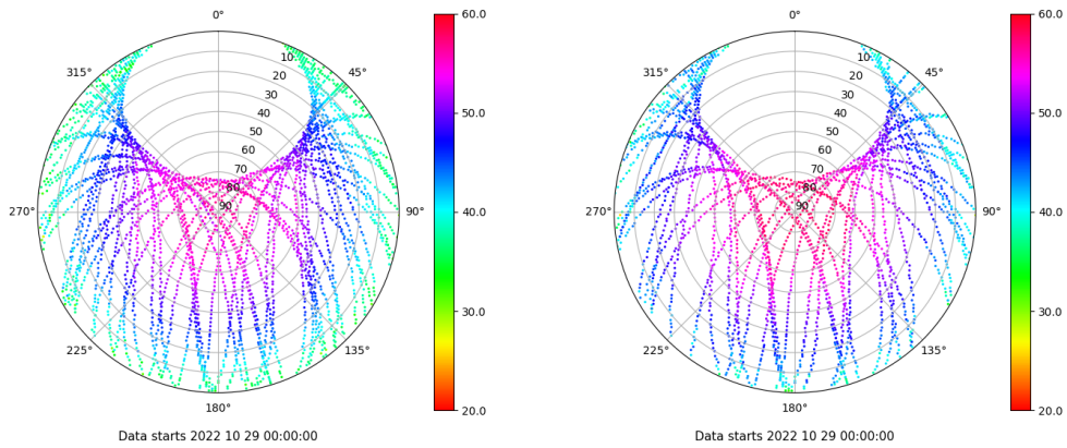
Skyplot for station XIXO. Signal to Noise S1C Data file XIXO00ESP_R_2022302.xtr Skyplot for station XIXO. Signal to Noise S2S Data file XIXO00ESP_R_2022302.xtr
