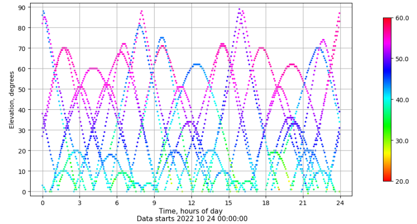
Time-elevation plot for station XIXO. Signal to Noise S1C Data file XIXO00ESP_R_2022297.xtr
