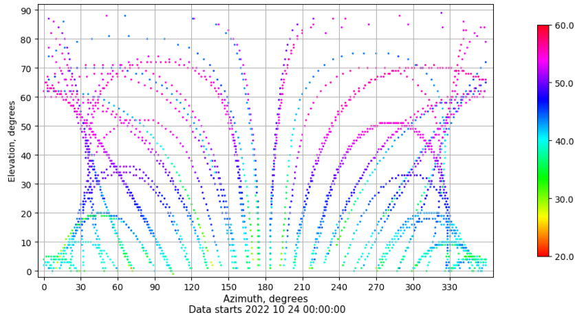
Azimuth-elevation plot for station XIXO. Signal to Noise S1C Data file XIXO00ESP_R_2022297.xtr
