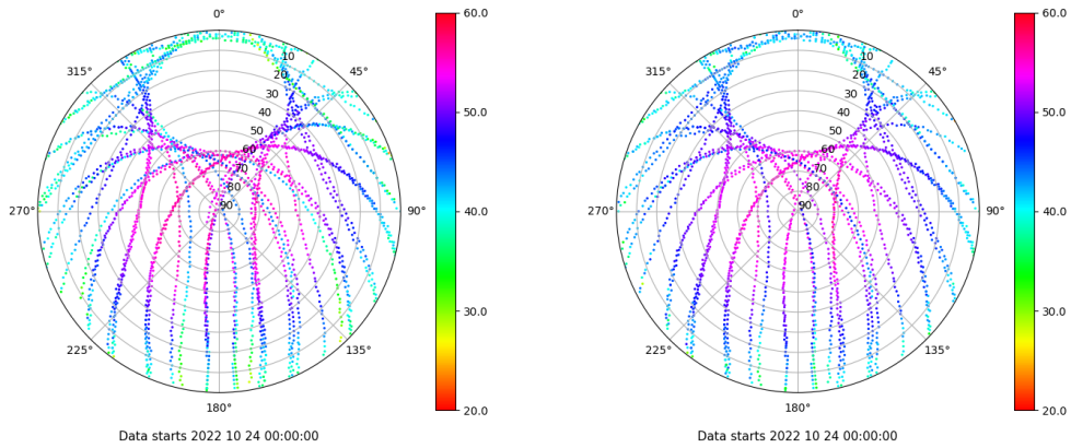
Skyplot for station XIXO. Signal to Noise S1C Data file XIXO00ESP_R_2022297.xtr Skyplot for station XIXO. Signal to Noise S2C Data file XIXO00ESP_R_2022297.xtr
