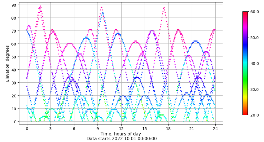
Time-elevation plot for station XIXO. Signal to Noise S1C Data file XIXO00ESP_R_2022274.xtr
