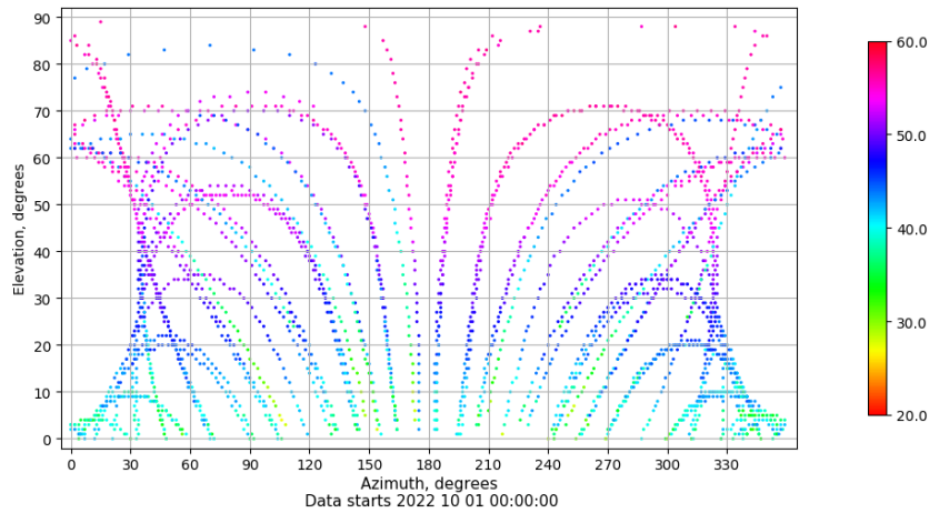
Azimuth-elevation plot for station XIXO. Signal to Noise S1C Data file XIXO00ESP_R_2022274.xtr
