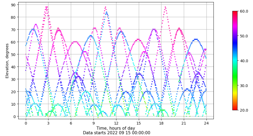
Time-elevation plot for station XIXO. Signal to Noise S1C Data file XIXO00ESP_R_2022258.xtr
