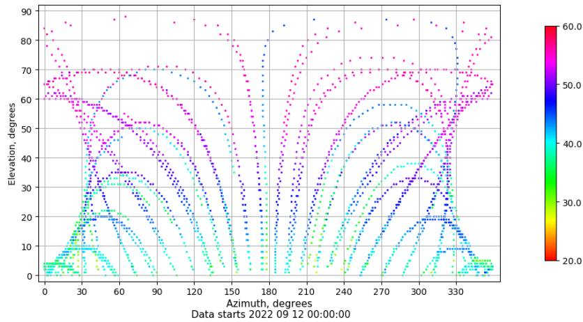
Azimuth-elevation plot for station XIXO. Signal to Noise S1C Data file XIXO00ESP_R_2022255.xtr
