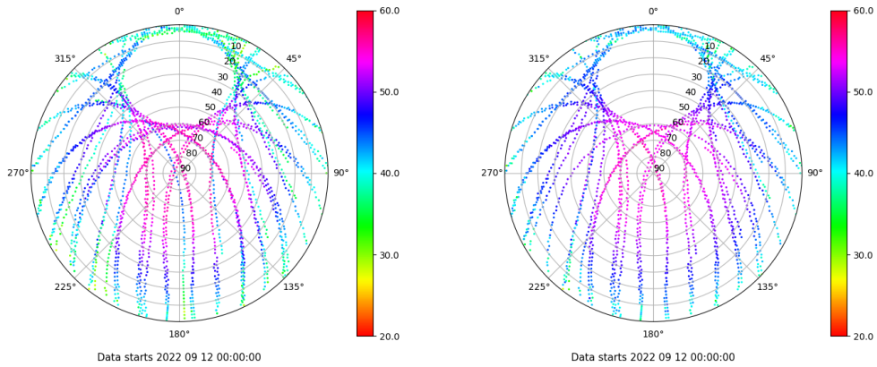
Skyplot for station XIXO. Signal to Noise S1C Data file XIXO00ESP_R_2022255.xtr Skyplot for station XIXO. Signal to Noise S2C Data file XIXO00ESP_R_2022255.xtr
