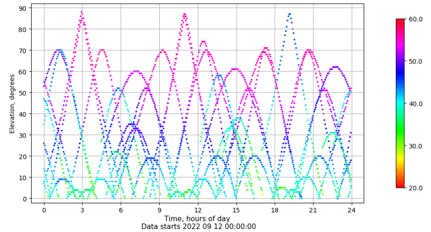
Time-elevation plot for station XIXO. Signal to Noise S1C Data file XIXO00ESP_R_2022255.xtr
