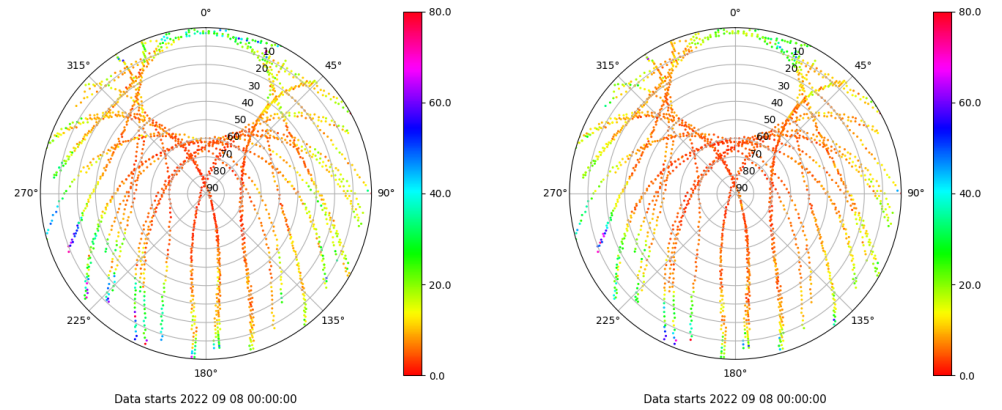
Skyplot for station XIXO. Parameter M1C Data file XIXO00ESP_R_2022251.xtr Skyplot for station XIXO. Parameter M2C Data file XIXO00ESP_R_2022251.xtr
