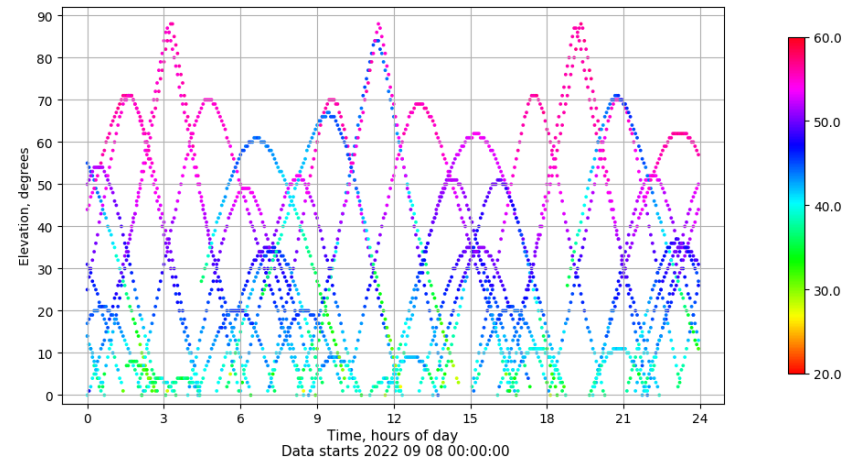
Time-elevation plot for station XIXO. Signal to Noise S1C Data file XIXO00ESP_R_2022251.xtr
