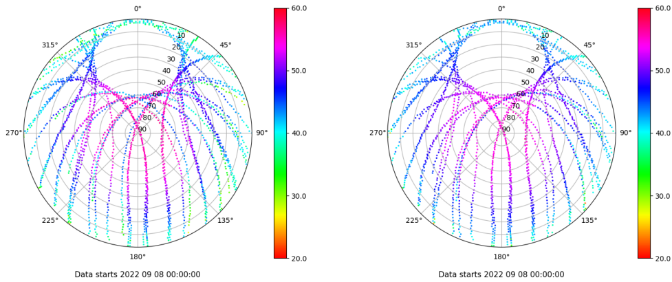
Skyplot for station XIXO. Signal to Noise S1C Data file XIXO00ESP_R_2022251.xtr Skyplot for station XIXO. Signal to Noise S2C Data file XIXO00ESP_R_2022251.xtr
