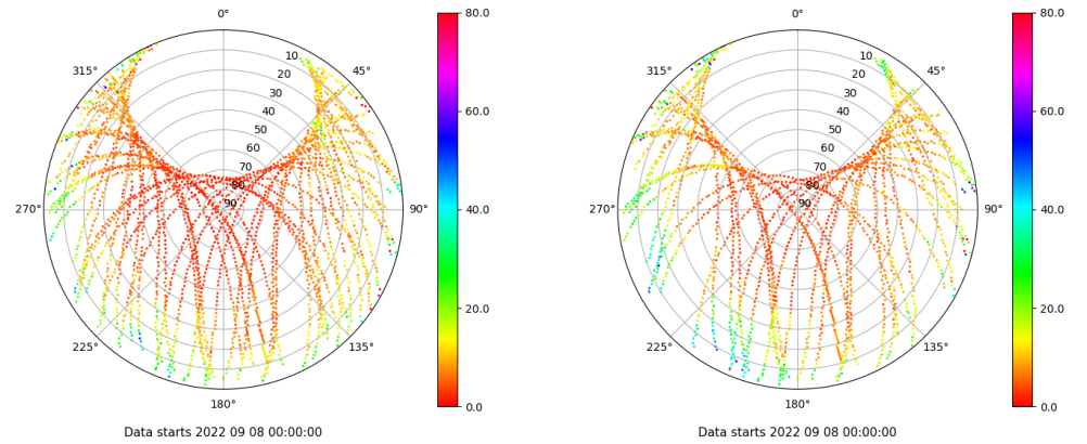
Skyplot for station XIXO. Parameter M1C Data file XIXO00ESP_R_2022251.xtr Skyplot for station XIXO. Parameter M2S Data file XIXO00ESP_R_2022251.xtr
