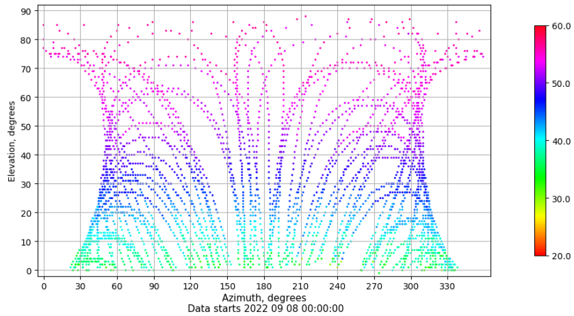
Azimuth-elevation plot for station XIXO. Signal to Noise S1C Data file XIXO00ESP_R_2022251.xtr
