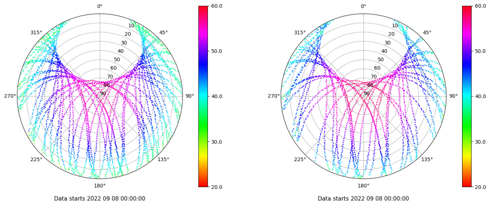
Skyplot for station XIXO. Signal to Noise S1C Data file XIXO00ESP_R_2022251.xtr Skyplot for station XIXO. Signal to Noise S2S Data file XIXO00ESP_R_2022251.xtr
