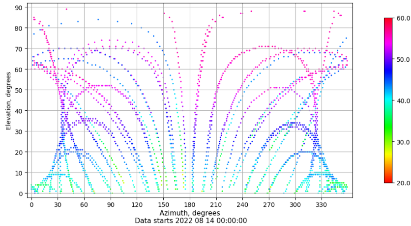
Azimuth-elevation plot for station XIXO. Signal to Noise S1C Data file XIXO00ESP_R_2022226.xtr
