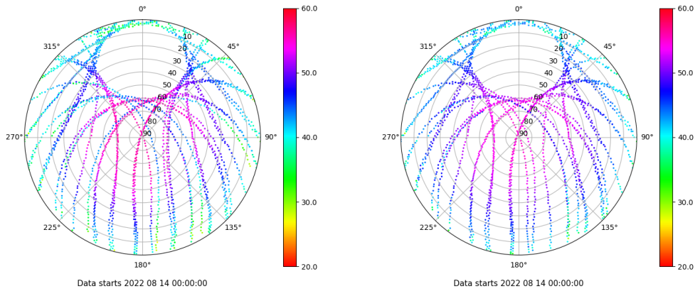
Skyplot for station XIXO. Signal to Noise S1C Data file XIXO00ESP_R_2022226.xtr Skyplot for station XIXO. Signal to Noise S2C Data file XIXO00ESP_R_2022226.xtr
