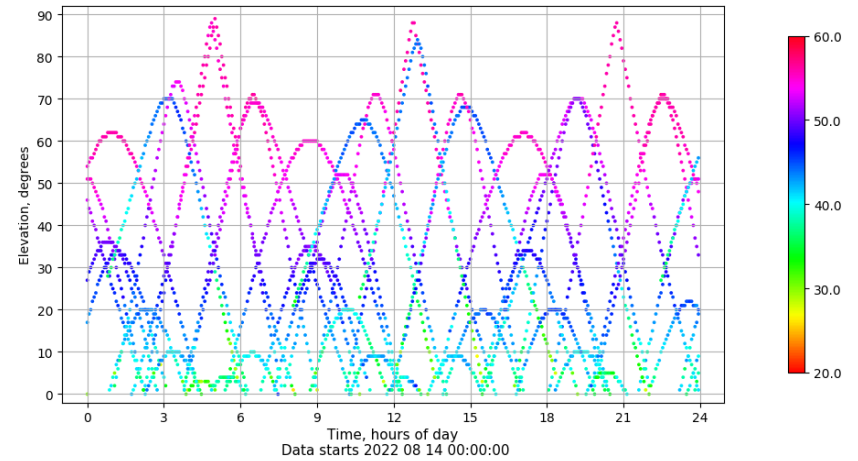
Time-elevation plot for station XIXO. Signal to Noise S1C Data file XIXO00ESP_R_2022226.xtr
