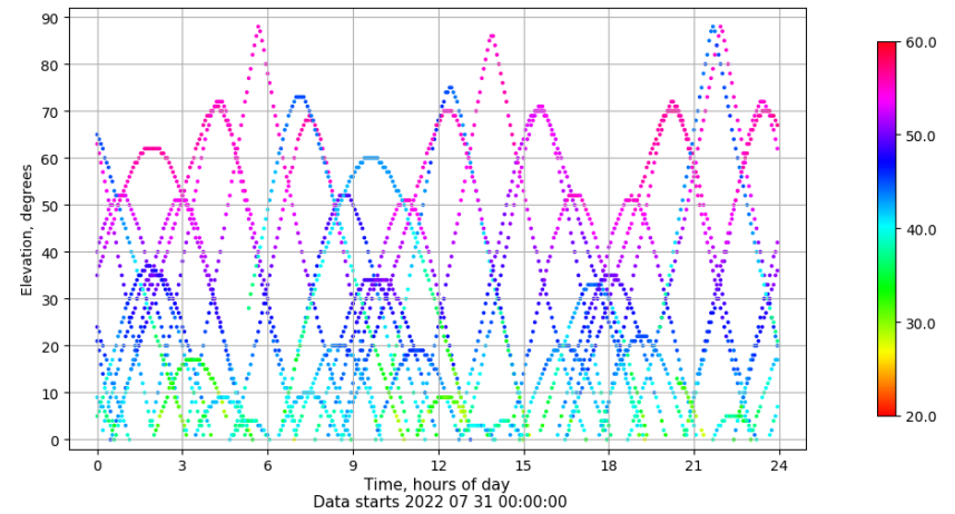
Time-elevation plot for station XIXO. Signal to Noise S1C Data file XIXO00ESP_R_2022212.xtr
