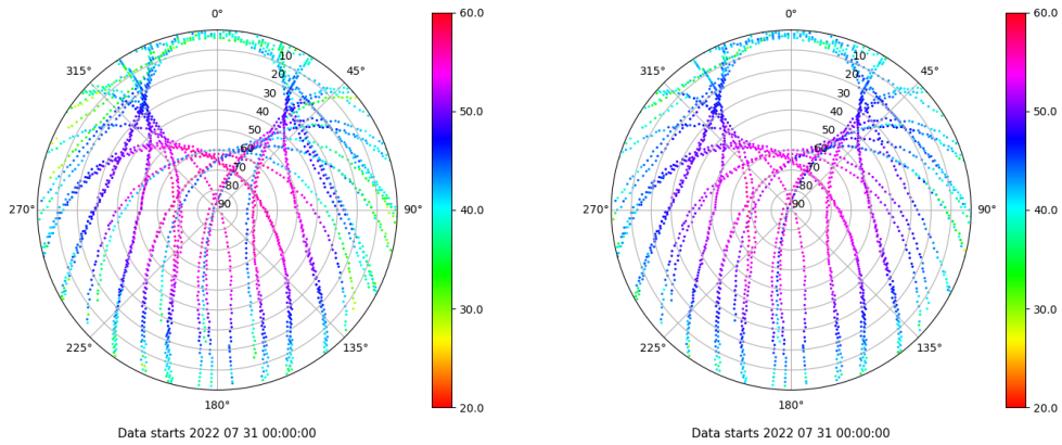
Skyplot for station XIXO. Signal to Noise S1C Data file XIXO00ESP_R_2022212.xtr Skyplot for station XIXO. Signal to Noise S2C Data file XIXO00ESP_R_2022212.xtr
