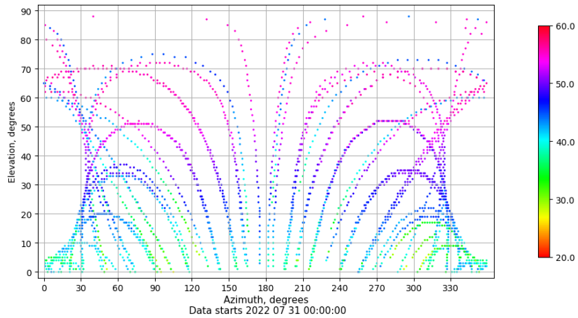
Azimuth-elevation plot for station XIXO. Signal to Noise S1C Data file XIXO00ESP_R_2022212.xtr
