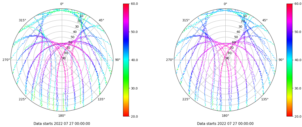
Skyplot for station XIXO. Signal to Noise S1C Data file XIXO00ESP_R_2022208.xtr Skyplot for station XIXO. Signal to Noise S2C Data file XIXO00ESP_R_2022208.xtr
