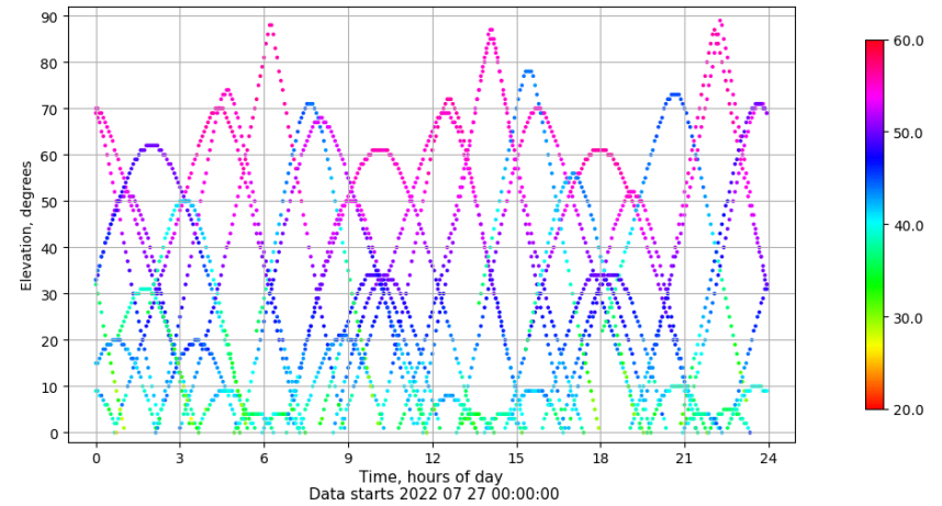
Time-elevation plot for station XIXO. Signal to Noise S1C Data file XIXO00ESP_R_2022208.xtr
