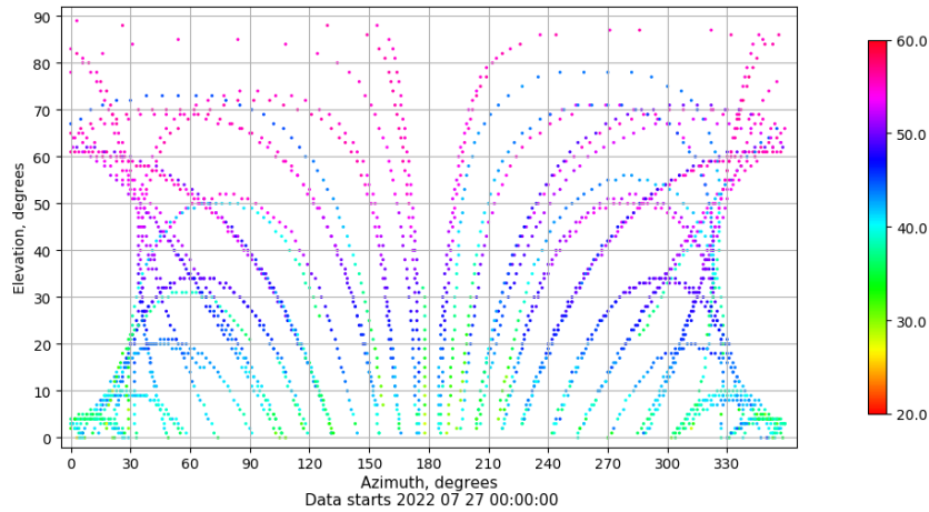
Azimuth-elevation plot for station XIXO. Signal to Noise S1C Data file XIXO00ESP_R_2022208.xtr
