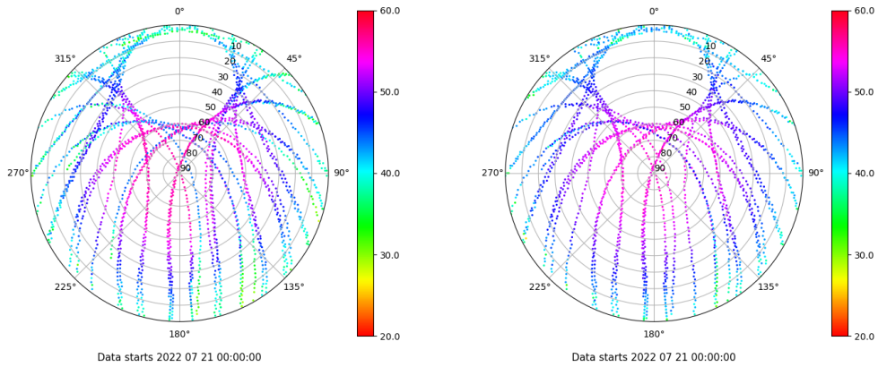
Skyplot for station XIXO. Signal to Noise S1C Data file XIXO00ESP_R_2022202.xtr Skyplot for station XIXO. Signal to Noise S2C Data file XIXO00ESP_R_2022202.xtr
