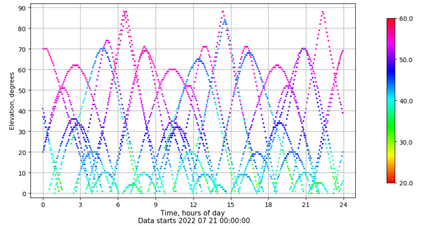
Time-elevation plot for station XIXO. Signal to Noise S1C Data file XIXO00ESP_R_2022202.xtr
