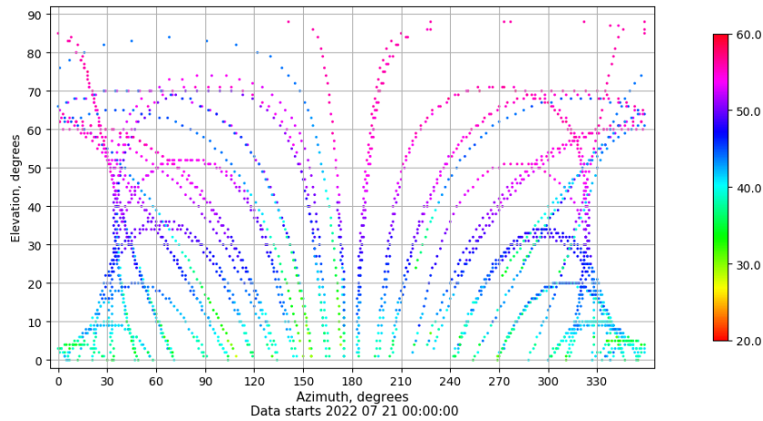
Azimuth-elevation plot for station XIXO. Signal to Noise S1C Data file XIXO00ESP_R_2022202.xtr
