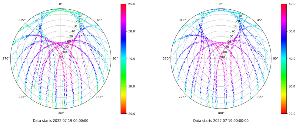
Skyplot for station XIXO. Signal to Noise S1C Data file XIXO00ESP_R_2022200.xtr Skyplot for station XIXO. Signal to Noise S2C Data file XIXO00ESP_R_2022200.xtr
