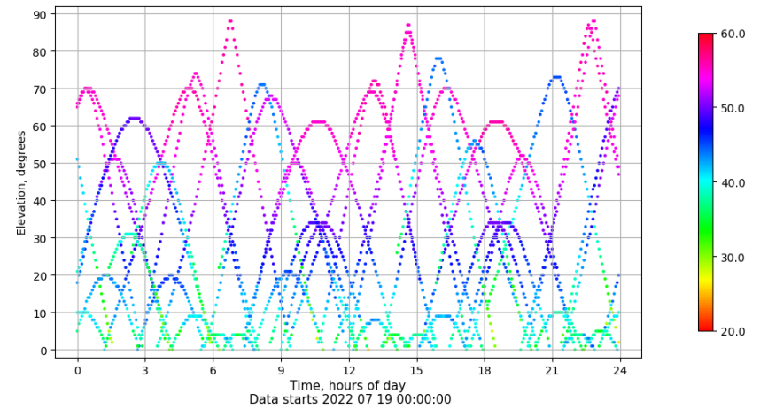
Time-elevation plot for station XIXO. Signal to Noise S1C Data file XIXO00ESP_R_2022200.xtr
