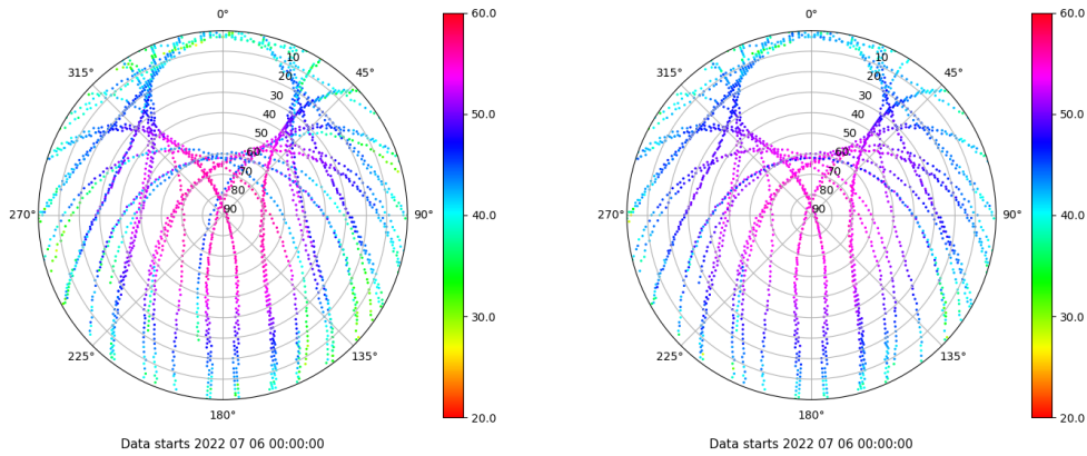
Skyplot for station XIXO. Signal to Noise S1C Data file XIXO00ESP_R_2022187.xtr Skyplot for station XIXO. Signal to Noise S2C Data file XIXO00ESP_R_2022187.xtr
