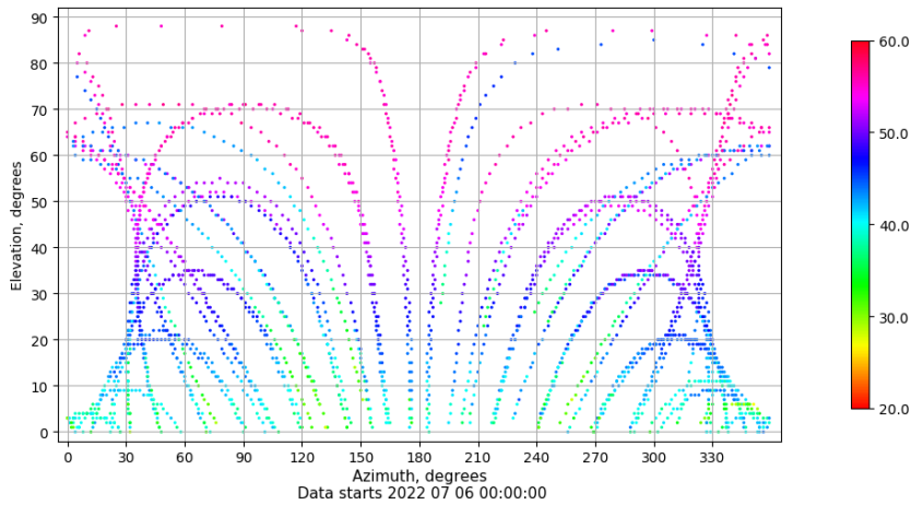
Azimuth-elevation plot for station XIXO. Signal to Noise S1C Data file XIXO00ESP_R_2022187.xtr
