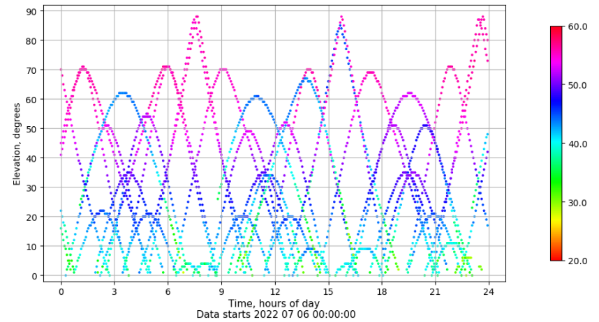
Time-elevation plot for station XIXO. Signal to Noise S1C Data file XIXO00ESP_R_2022187.xtr
