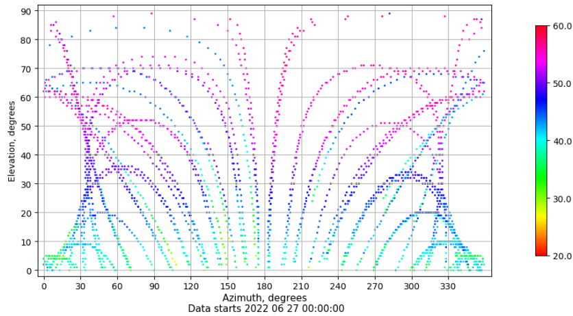
Azimuth-elevation plot for station XIXO. Signal to Noise S1C Data file XIXO00ESP_R_2022178.xtr
