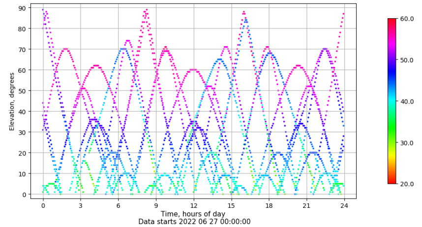
Time-elevation plot for station XIXO. Signal to Noise S1C Data file XIXO00ESP_R_2022178.xtr
