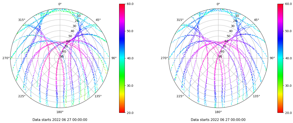
Skyplot for station XIXO. Signal to Noise S1C Data file XIXO00ESP_R_2022178.xtr Skyplot for station XIXO. Signal to Noise S2C Data file XIXO00ESP_R_2022178.xtr
