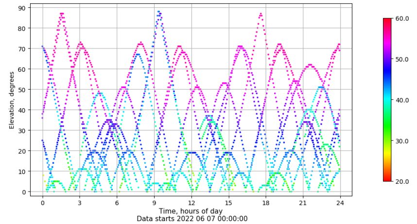
Time-elevation plot for station XIXO. Signal to Noise S1C Data file XIXO00ESP_R_2022158.xtr
