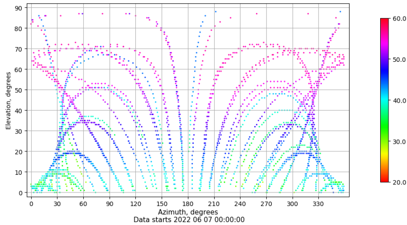
Azimuth-elevation plot for station XIXO. Signal to Noise S1C Data file XIXO00ESP_R_2022158.xtr
