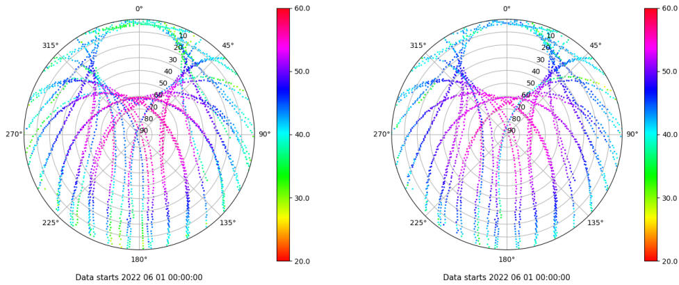
Skyplot for station XIXO. Signal to Noise S1C Data file XIXO00ESP_R_2022152.xtr Skyplot for station XIXO. Signal to Noise S2C Data file XIXO00ESP_R_2022152.xtr
