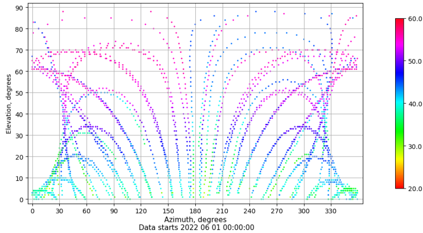
Azimuth-elevation plot for station XIXO. Signal to Noise S1C Data file XIXO00ESP_R_2022152.xtr
