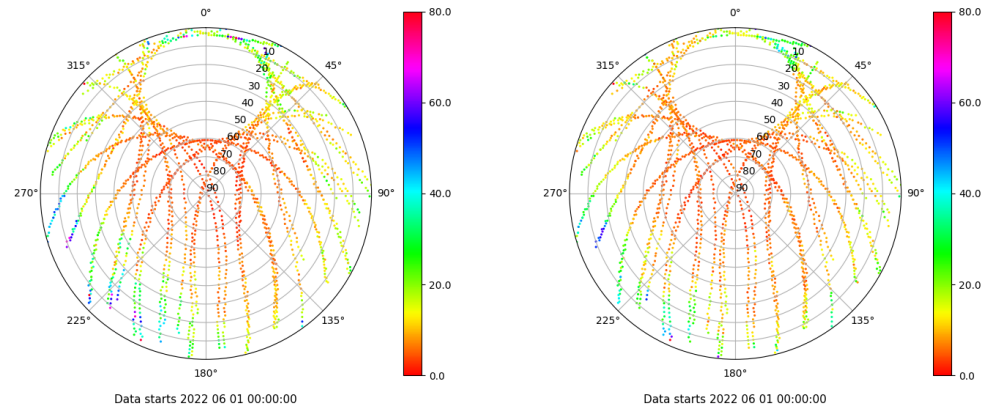
Skyplot for station XIXO. Parameter M1C Data file XIXO00ESP_R_2022152.xtr Skyplot for station XIXO. Parameter M2C Data file XIXO00ESP_R_2022152.xtr
