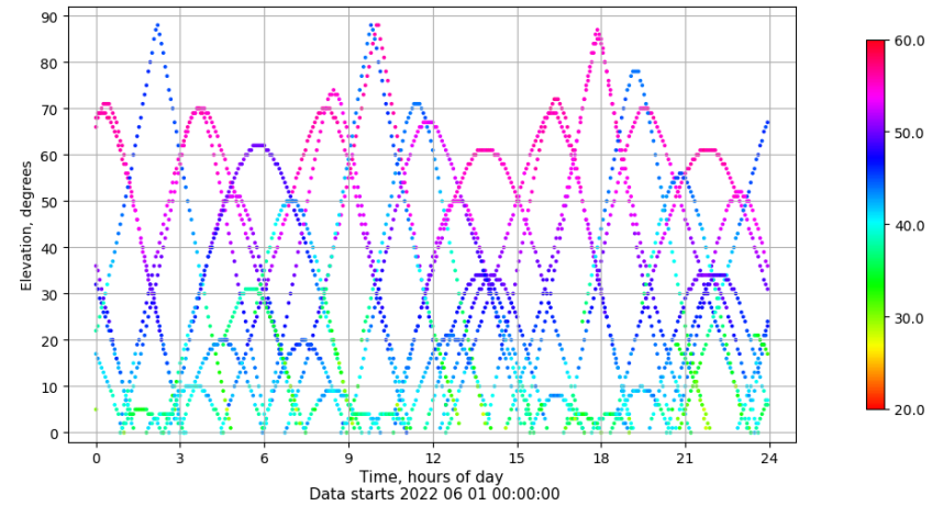
Time-elevation plot for station XIXO. Signal to Noise S1C Data file XIXO00ESP_R_2022152.xtr
