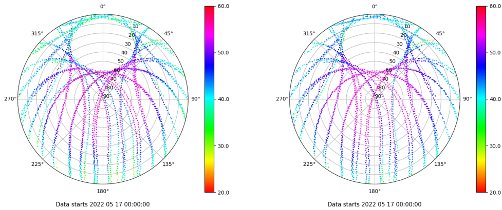
Skyplot for station XIXO. Signal to Noise S1C Data file XIXO00ESP_R_2022137.xtr Skyplot for station XIXO. Signal to Noise S2C Data file XIXO00ESP_R_2022137.xtr
