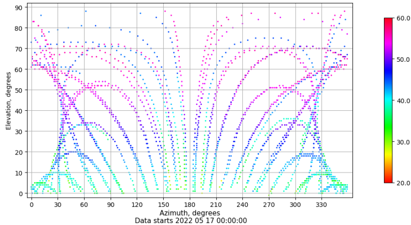
Azimuth-elevation plot for station XIXO. Signal to Noise S1C Data file XIXO00ESP_R_2022137.xtr
