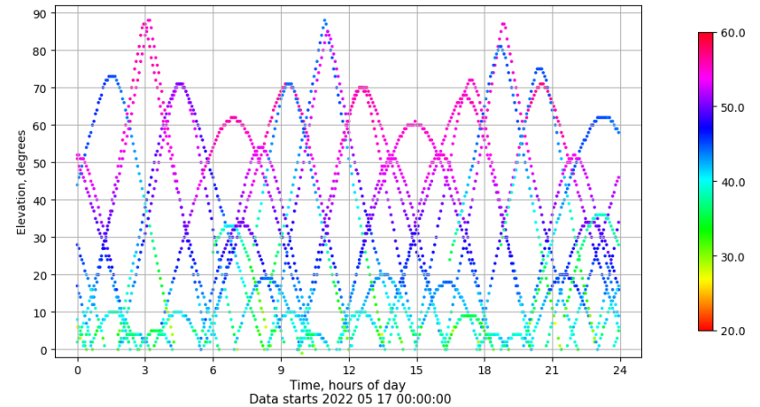
Time-elevation plot for station XIXO. Signal to Noise S1C Data file XIXO00ESP_R_2022137.xtr
