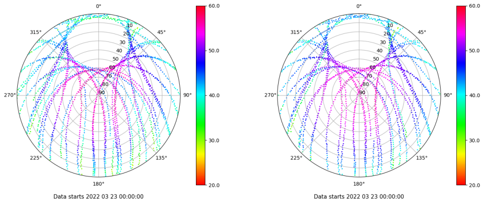
Skyplot for station XIXO. Signal to Noise S1C Data file XIXO00ESP_R_2022082.xtr Skyplot for station XIXO. Signal to Noise S2C Data file XIXO00ESP_R_2022082.xtr
