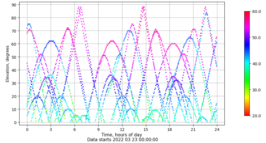
Time-elevation plot for station XIXO. Signal to Noise S1C Data file XIXO00ESP_R_2022082.xtr
