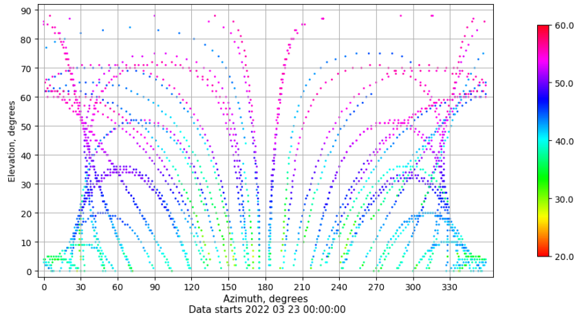
Azimuth-elevation plot for station XIXO. Signal to Noise S1C Data file XIXO00ESP_R_2022082.xtr
