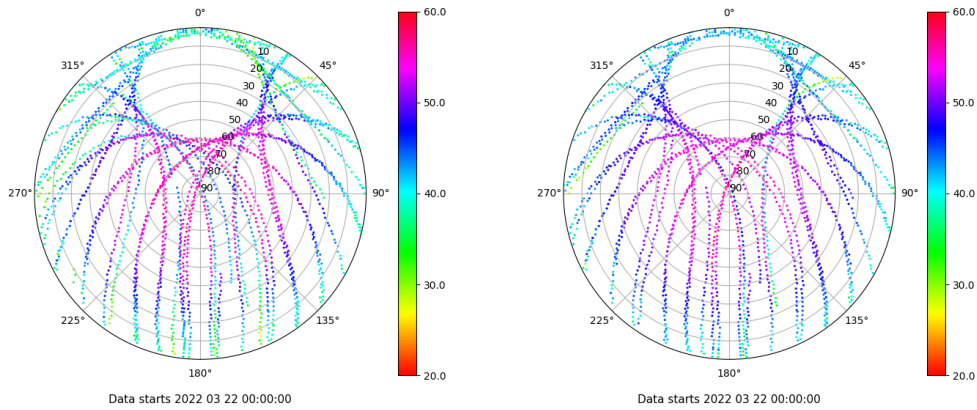
Skyplot for station XIXO. Signal to Noise S1C Data file XIXO00ESP_R_2022081.xtr Skyplot for station XIXO. Signal to Noise S2C Data file XIXO00ESP_R_2022081.xtr
