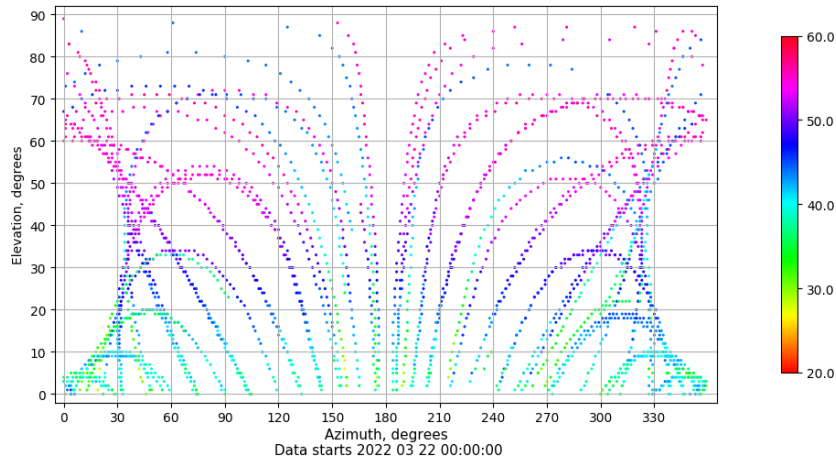
Azimuth-elevation plot for station XIXO. Signal to Noise S1C Data file XIXO00ESP_R_2022081.xtr
