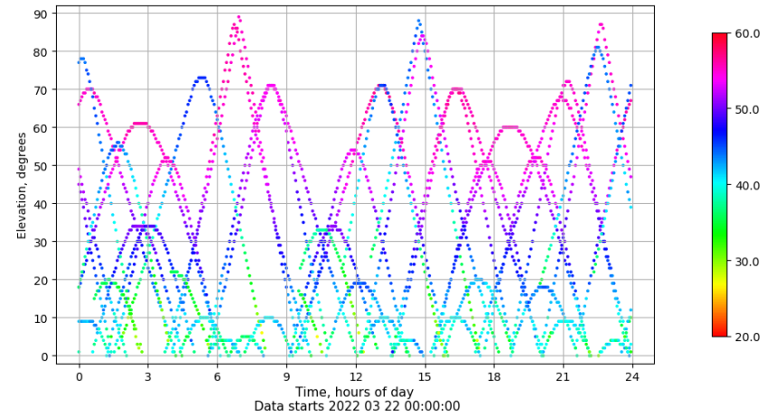
Time-elevation plot for station XIXO. Signal to Noise S1C Data file XIXO00ESP_R_2022081.xtr
