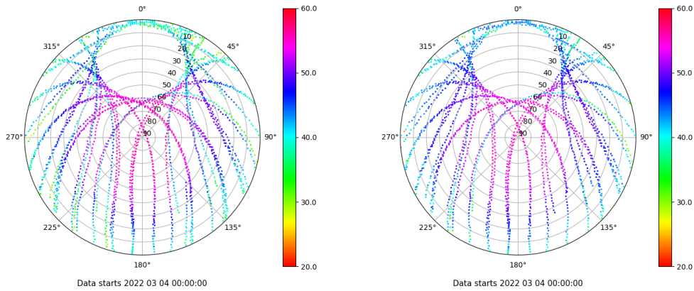
Skyplot for station XIXO. Signal to Noise S1C Data file XIXO00ESP_R_2022063.xtr Skyplot for station XIXO. Signal to Noise S2C Data file XIXO00ESP_R_2022063.xtr
