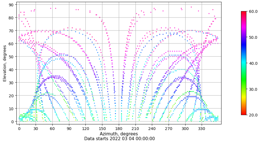
Azimuth-elevation plot for station XIXO. Signal to Noise S1C Data file XIXO00ESP_R_2022063.xtr
