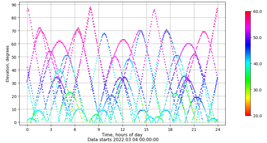
Time-elevation plot for station XIXO. Signal to Noise S1C Data file XIXO00ESP_R_2022063.xtr
