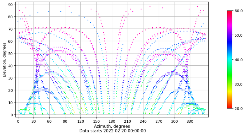
Azimuth-elevation plot for station XIXO. Signal to Noise S1C Data file XIXO00ESP_R_2022051.xtr
