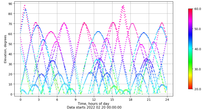
Time-elevation plot for station XIXO. Signal to Noise S1C Data file XIXO00ESP_R_2022051.xtr
