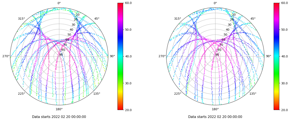
Skyplot for station XIXO. Signal to Noise S1C Data file XIXO00ESP_R_2022051.xtr Skyplot for station XIXO. Signal to Noise S2C Data file XIXO00ESP_R_2022051.xtr
