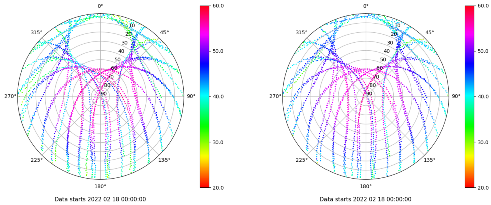
Skyplot for station XIXO. Signal to Noise S1C Data file XIXO00ESP_R_2022049.xtr Skyplot for station XIXO. Signal to Noise S2C Data file XIXO00ESP_R_2022049.xtr
