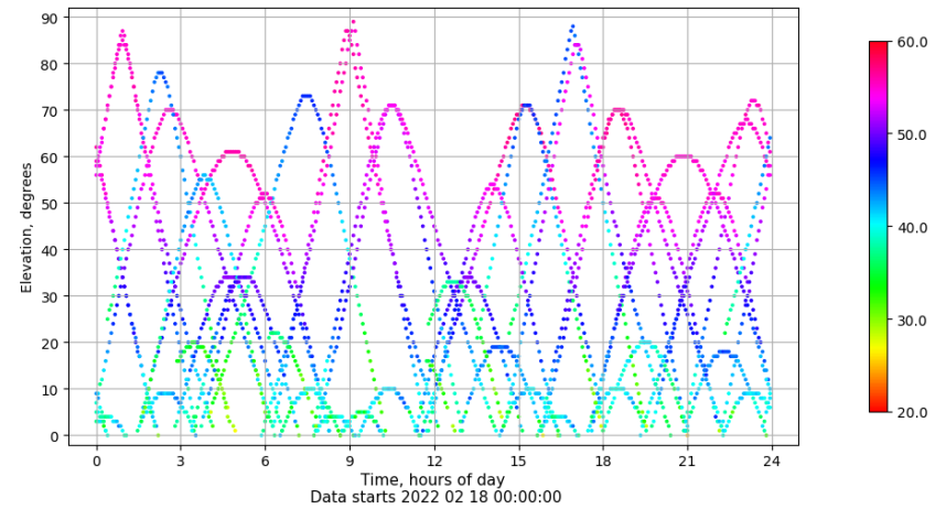
Time-elevation plot for station XIXO. Signal to Noise S1C Data file XIXO00ESP_R_2022049.xtr
