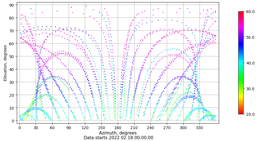
Azimuth-elevation plot for station XIXO. Signal to Noise S1C Data file XIXO00ESP_R_2022049.xtr
