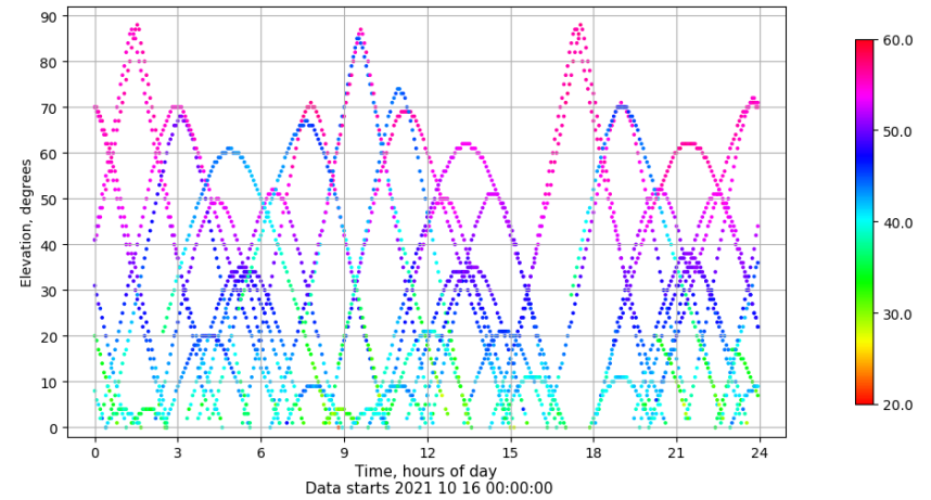
Time-elevation plot for station XIXO. Signal to Noise S1C Data file XIXO00ESP_R_2021289.xtr
