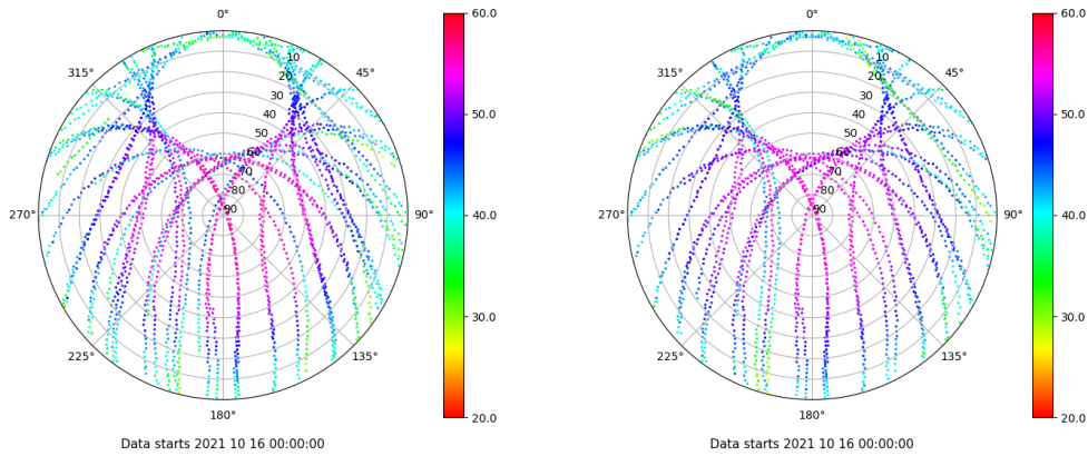
Skyplot for station XIXO. Signal to Noise S1C Data file XIXO00ESP_R_2021289.xtr Skyplot for station XIXO. Signal to Noise S2C Data file XIXO00ESP_R_2021289.xtr
