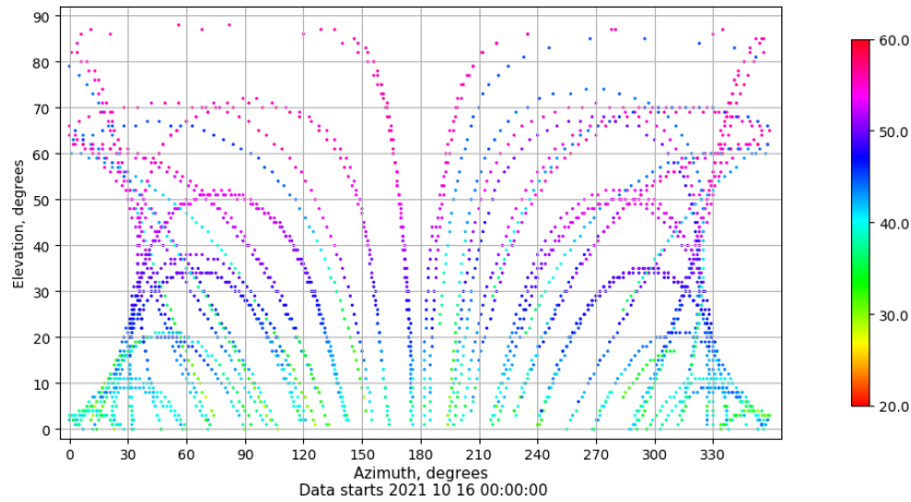
Azimuth-elevation plot for station XIXO. Signal to Noise S1C Data file XIXO00ESP_R_2021289.xtr
