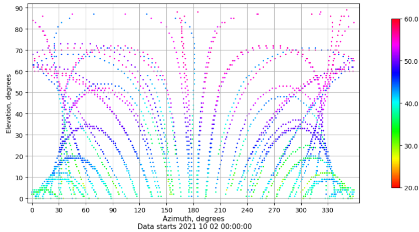
Azimuth-elevation plot for station XIXO. Signal to Noise S1C Data file XIXO00ESP_R_2021275.xtr
