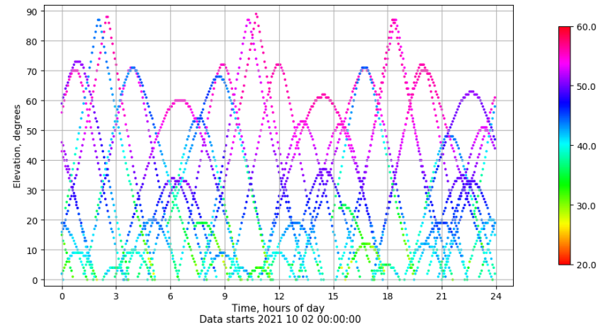
Time-elevation plot for station XIXO. Signal to Noise S1C Data file XIXO00ESP_R_2021275.xtr
