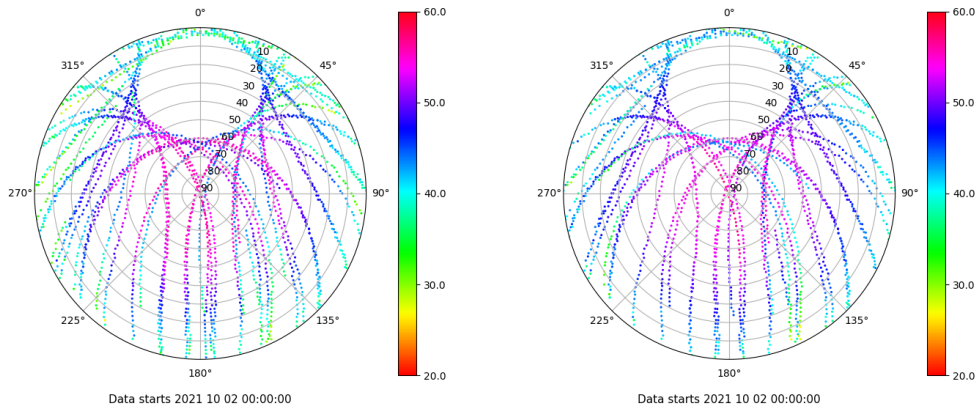
Skyplot for station XIXO. Signal to Noise S1C Data file XIXO00ESP_R_2021275.xtr Skyplot for station XIXO. Signal to Noise S2C Data file XIXO00ESP_R_2021275.xtr
