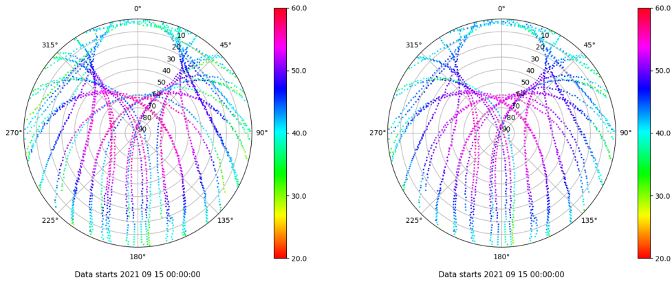
Skyplot for station XIXO. Signal to Noise S1C Data file XIXO00ESP_R_2021258.xtr Skyplot for station XIXO. Signal to Noise S2C Data file XIXO00ESP_R_2021258.xtr
