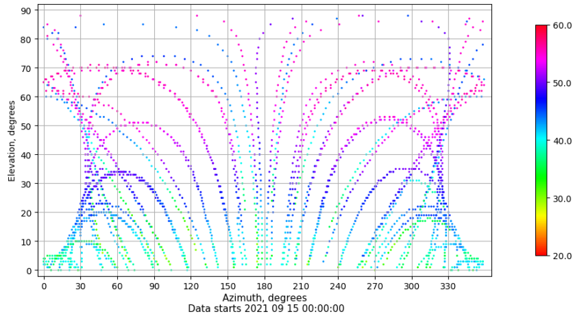
Azimuth-elevation plot for station XIXO. Signal to Noise S1C Data file XIXO00ESP_R_2021258.xtr
