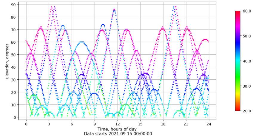
Time-elevation plot for station XIXO. Signal to Noise S1C Data file XIXO00ESP_R_2021258.xtr
