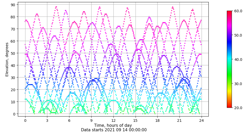
Time-elevation plot for station XIXO. Signal to Noise S1C Data file XIXO00ESP_R_2021257.xtr
