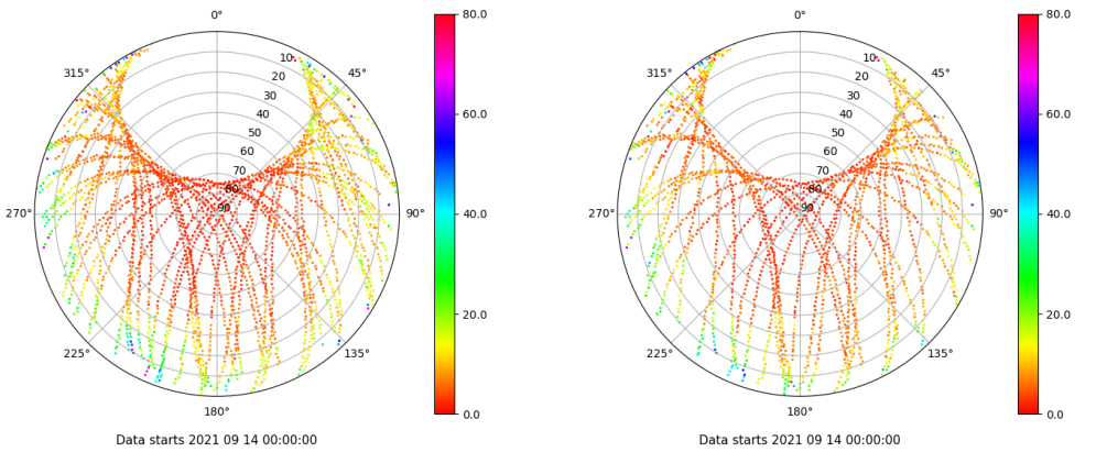
Skyplot for station XIXO. Parameter M1C Data file XIXO00ESP_R_2021257.xtr Skyplot for station XIXO. Parameter M2S Data file XIXO00ESP_R_2021257.xtr
