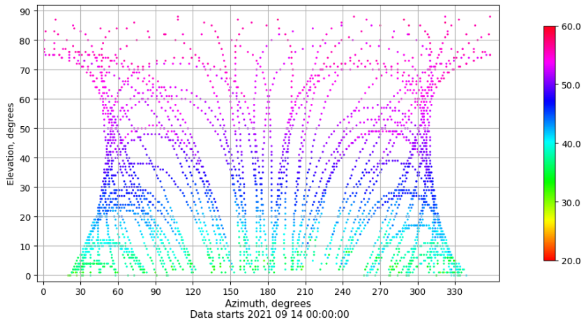
Azimuth-elevation plot for station XIXO. Signal to Noise S1C Data file XIXO00ESP_R_2021257.xtr
