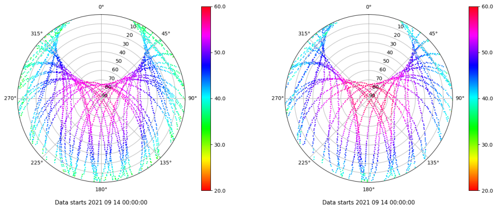
Skyplot for station XIXO. Signal to Noise S1C Data file XIXO00ESP_R_2021257.xtr Skyplot for station XIXO. Signal to Noise S2S Data file XIXO00ESP_R_2021257.xtr
