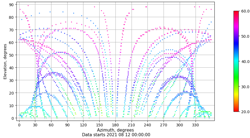
Azimuth-elevation plot for station XIXO. Signal to Noise S1C Data file XIXO00ESP_R_2021224.xtr
