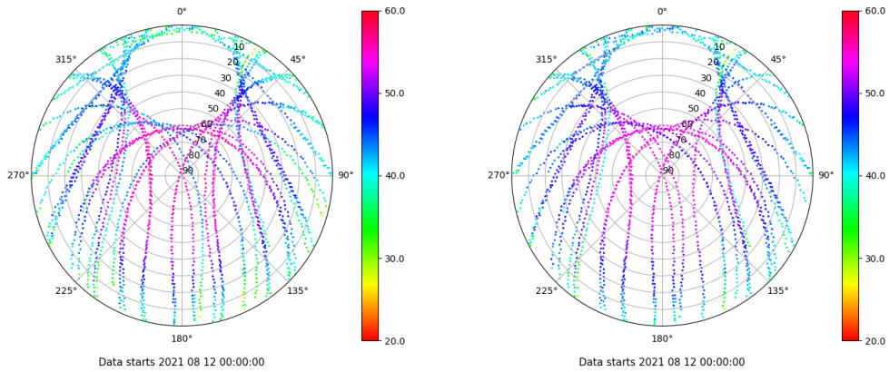
Skyplot for station XIXO. Signal to Noise S1C Data file XIXO00ESP_R_2021224.xtr Skyplot for station XIXO. Signal to Noise S2C Data file XIXO00ESP_R_2021224.xtr
