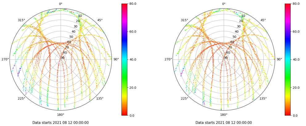
Skyplot for station XIXO. Parameter M1C Data file XIXO00ESP_R_2021224.xtr Skyplot for station XIXO. Parameter M2C Data file XIXO00ESP_R_2021224.xtr
