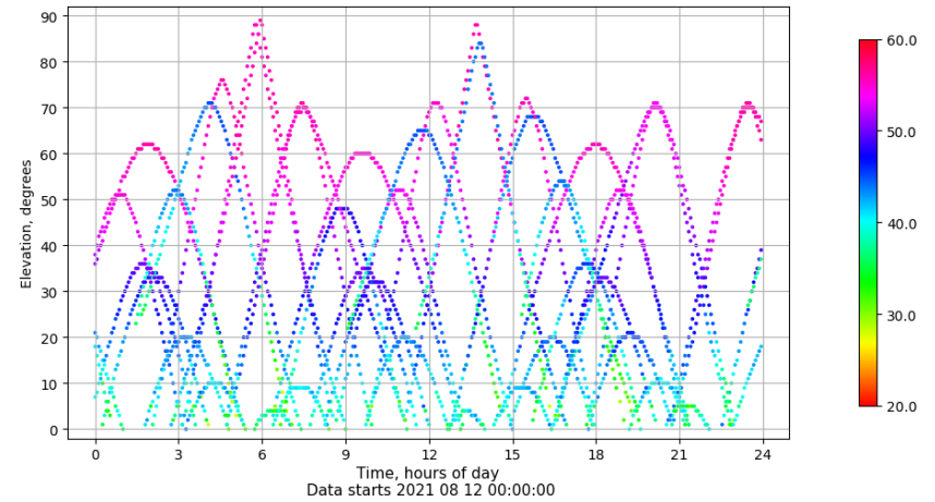
Time-elevation plot for station XIXO. Signal to Noise S1C Data file XIXO00ESP_R_2021224.xtr
