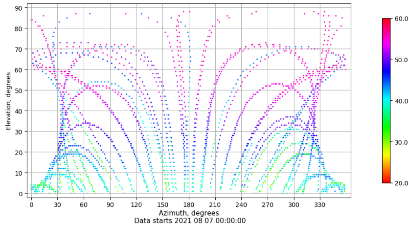
Azimuth-elevation plot for station XIXO. Signal to Noise S1C Data file XIXO00ESP_R_2021219.xtr
