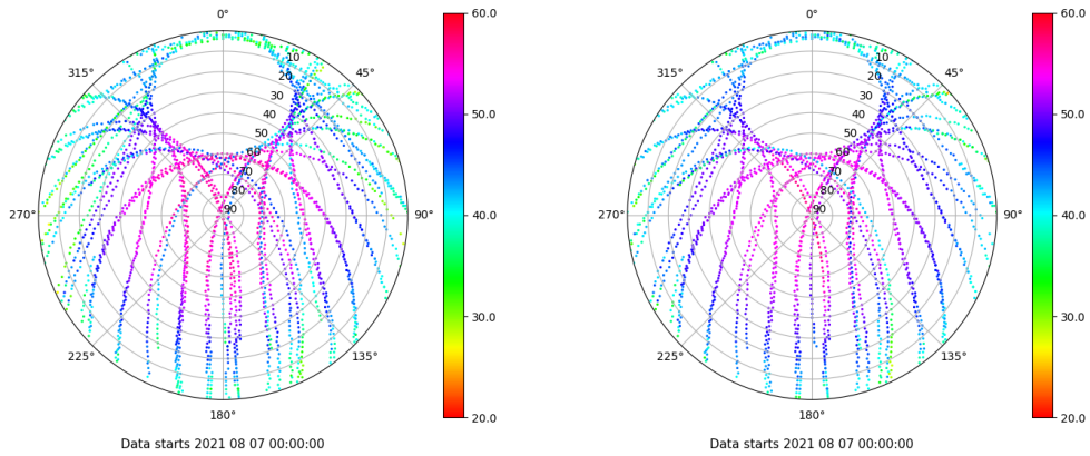
Skyplot for station XIXO. Signal to Noise S1C Data file XIXO00ESP_R_2021219.xtr Skyplot for station XIXO. Signal to Noise S2C Data file XIXO00ESP_R_2021219.xtr
