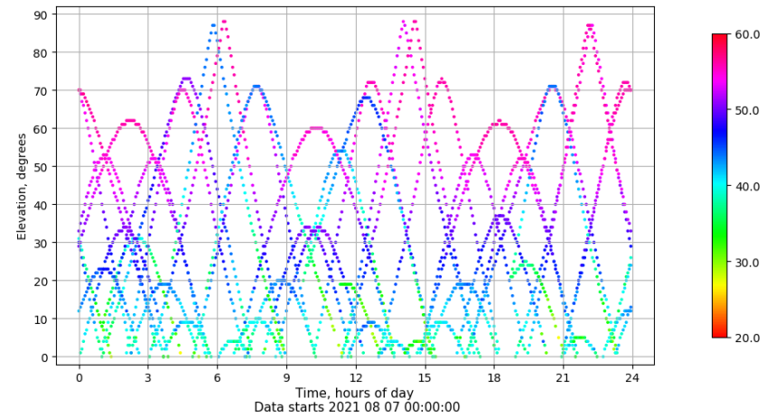
Time-elevation plot for station XIXO. Signal to Noise S1C Data file XIXO00ESP_R_2021219.xtr
