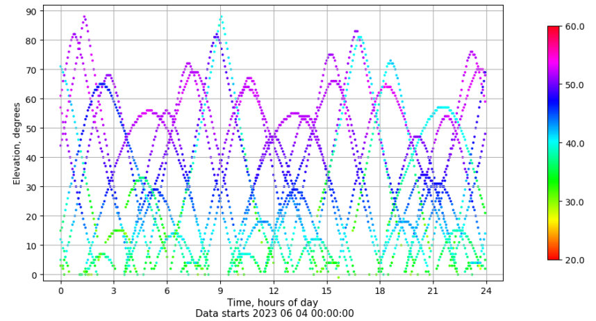
Time-elevation plot for station VILH. Signal to Noise S1C Data file VILH00ESP_R_2023155.xtr
