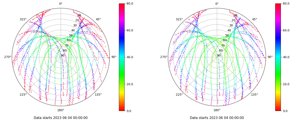
Skyplot for station VILH. Parameter M1C Data file VILH00ESP_R_2023155.xtr Skyplot for station VILH. Parameter M2C Data file VILH00ESP_R_2023155.xtr
