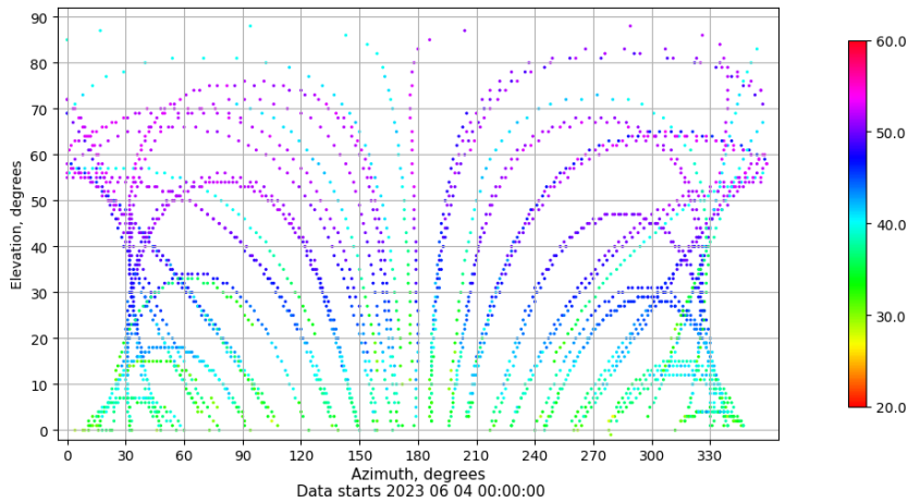
Azimuth-elevation plot for station VILH. Signal to Noise S1C Data file VILH00ESP_R_2023155.xtr
