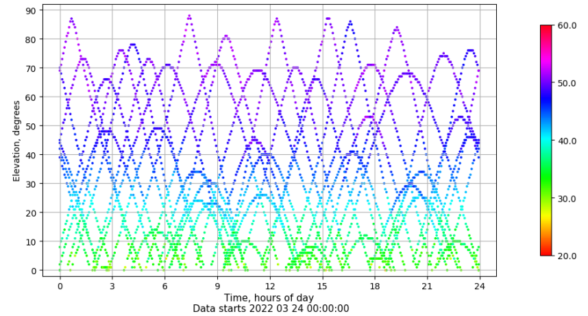
Time-elevation plot for station VILH. Signal to Noise S1C Data file VILH00ESP_R_2022083.xtr
