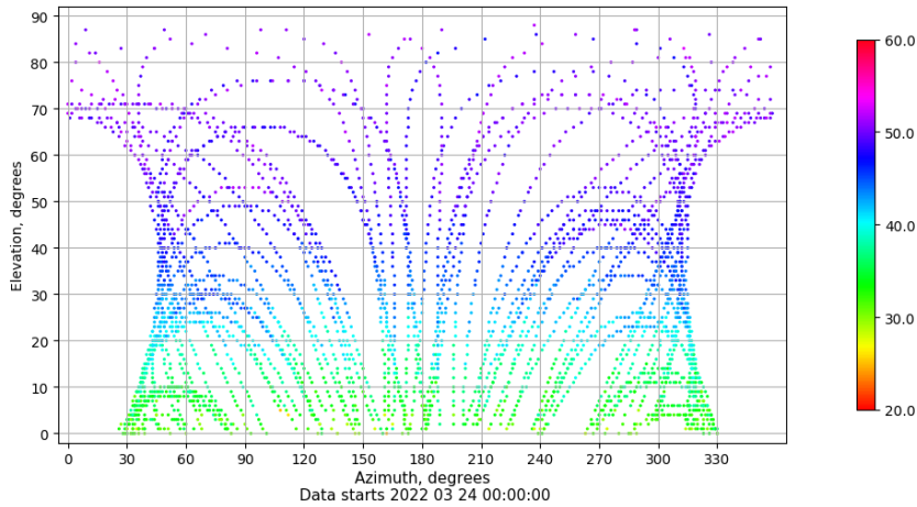
Azimuth-elevation plot for station VILH. Signal to Noise S1C Data file VILH00ESP_R_2022083.xtr
