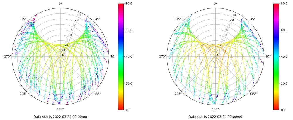
Skyplot for station VILH. Parameter M1C Data file VILH00ESP_R_2022083.xtr Skyplot for station VILH. Parameter M2X Data file VILH00ESP_R_2022083.xtr
