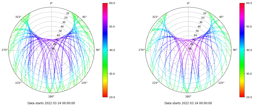
Skyplot for station VILH. Signal to Noise S1C Data file VILH00ESP_R_2022083.xtr Skyplot for station VILH. Signal to Noise S2X Data file VILH00ESP_R_2022083.xtr
