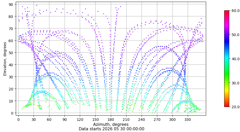
Azimuth-elevation plot for station VIGO. Signal to Noise S1C Data file VIGO00ESP_R_2026150.xtr
