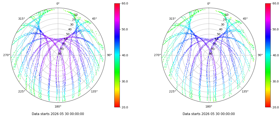
Skyplot for station VIGO. Signal to Noise S1C Data file VIGO00ESP_R_2026150.xtr Skyplot for station VIGO. Signal to Noise S2C Data file VIGO00ESP_R_2026150.xtr
