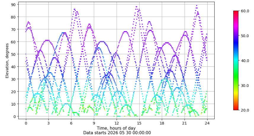
Time-elevation plot for station VIGO. Signal to Noise S1C Data file VIGO00ESP_R_2026150.xtr
