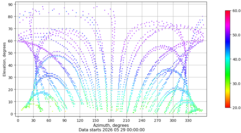
Azimuth-elevation plot for station VIGO. Signal to Noise S1C Data file VIGO00ESP_R_2026149.xtr
