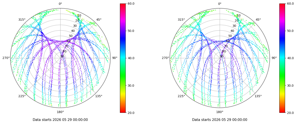
Skyplot for station VIGO. Signal to Noise S1C Data file VIGO00ESP_R_2026149.xtr Skyplot for station VIGO. Signal to Noise S2C Data file VIGO00ESP_R_2026149.xtr
