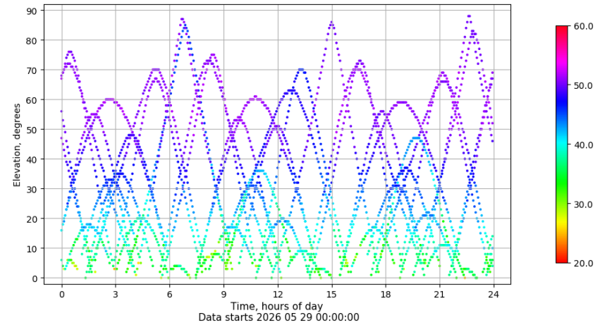
Time-elevation plot for station VIGO. Signal to Noise S1C Data file VIGO00ESP_R_2026149.xtr
