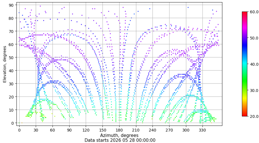
Azimuth-elevation plot for station VIGO. Signal to Noise S1C Data file VIGO00ESP_R_2026148.xtr
