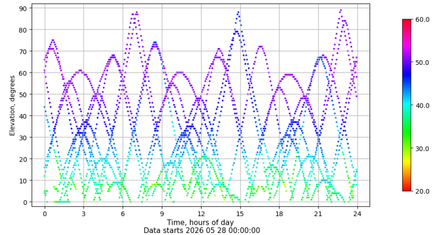
Time-elevation plot for station VIGO. Signal to Noise S1C Data file VIGO00ESP_R_2026148.xtr
