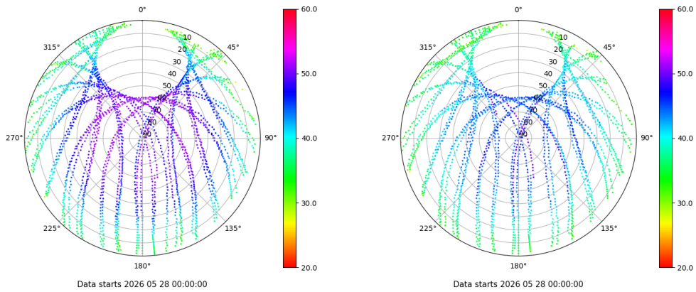
Skyplot for station VIGO. Signal to Noise S1C Data file VIGO00ESP_R_2026148.xtr Skyplot for station VIGO. Signal to Noise S2C Data file VIGO00ESP_R_2026148.xtr
