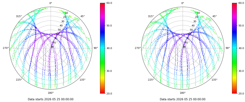
Skyplot for station VIGO. Signal to Noise S1C Data file VIGO00ESP_R_2026145.xtr Skyplot for station VIGO. Signal to Noise S2C Data file VIGO00ESP_R_2026145.xtr
