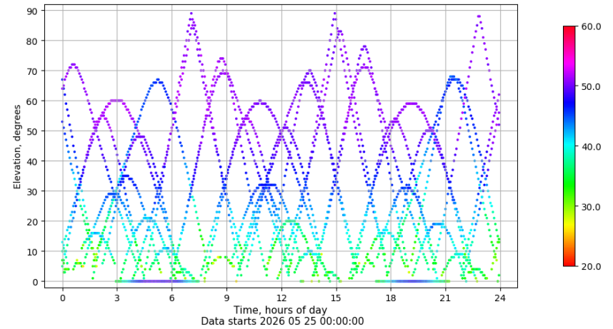
Time-elevation plot for station VIGO. Signal to Noise S1C Data file VIGO00ESP_R_2026145.xtr
