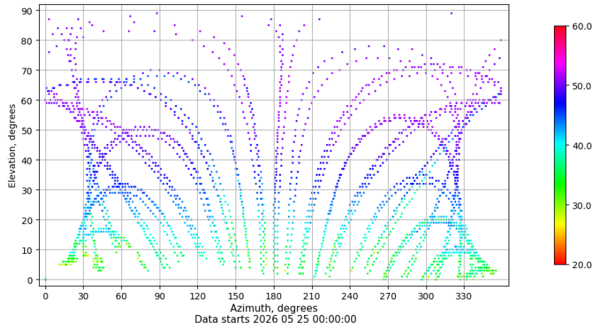
Azimuth-elevation plot for station VIGO. Signal to Noise S1C Data file VIGO00ESP_R_2026145.xtr
