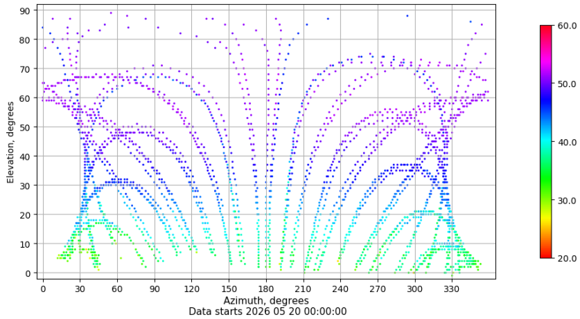
Azimuth-elevation plot for station VIGO. Signal to Noise S1C Data file VIGO00ESP_R_2026140.xtr
