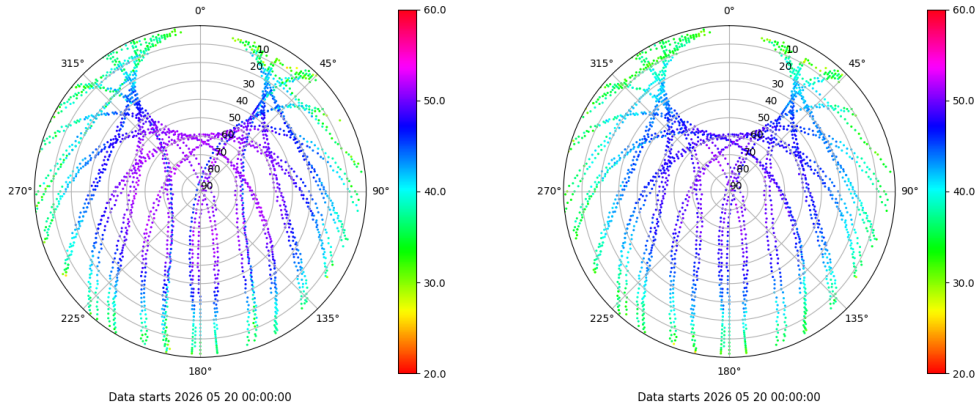
Skyplot for station VIGO. Signal to Noise S1C Data file VIGO00ESP_R_2026140.xtr Skyplot for station VIGO. Signal to Noise S2C Data file VIGO00ESP_R_2026140.xtr
