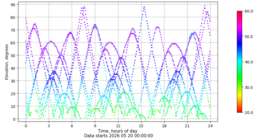
Time-elevation plot for station VIGO. Signal to Noise S1C Data file VIGO00ESP_R_2026140.xtr
