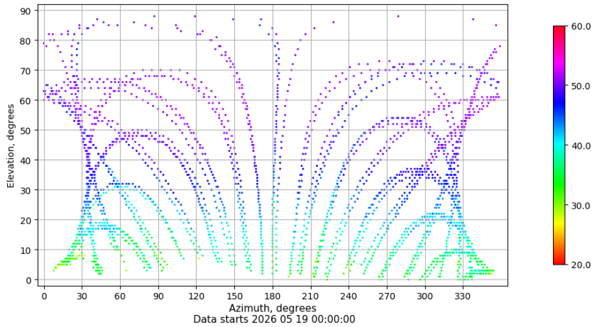
Azimuth-elevation plot for station VIGO. Signal to Noise S1C Data file VIGO00ESP_R_2026139.xtr
