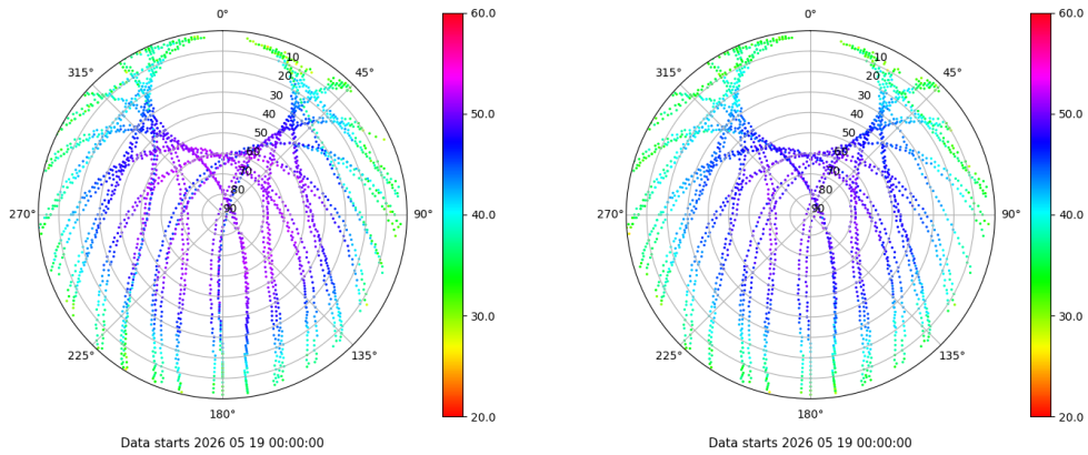
Skyplot for station VIGO. Signal to Noise S1C Data file VIGO00ESP_R_2026139.xtr Skyplot for station VIGO. Signal to Noise S2C Data file VIGO00ESP_R_2026139.xtr
