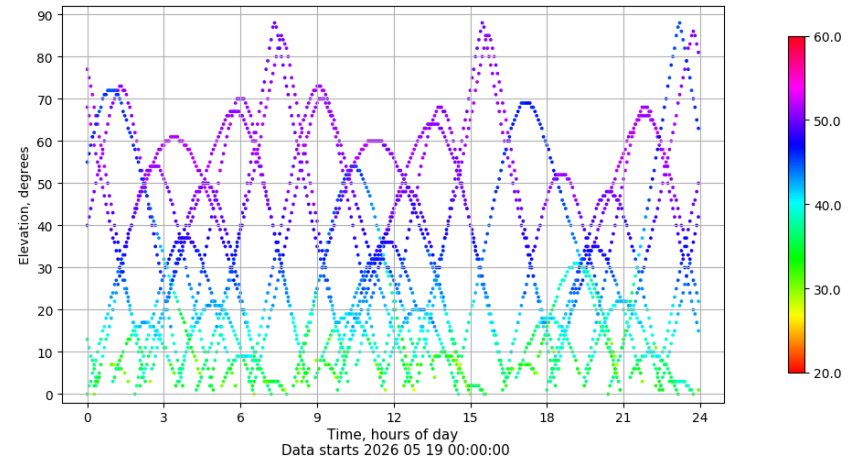
Time-elevation plot for station VIGO. Signal to Noise S1C Data file VIGO00ESP_R_2026139.xtr
