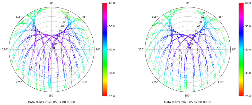
Skyplot for station VIGO. Signal to Noise S1C Data file VIGO00ESP_R_2026127.xtr Skyplot for station VIGO. Signal to Noise S2C Data file VIGO00ESP_R_2026127.xtr
