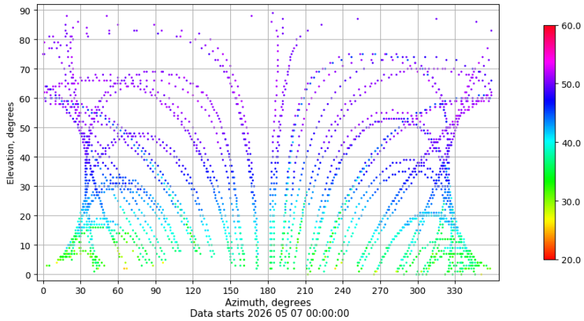
Azimuth-elevation plot for station VIGO. Signal to Noise S1C Data file VIGO00ESP_R_2026127.xtr
