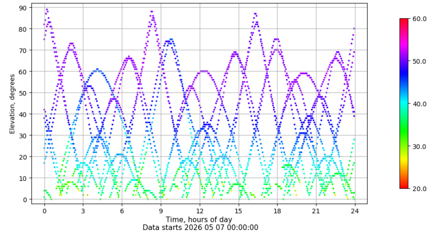
Time-elevation plot for station VIGO. Signal to Noise S1C Data file VIGO00ESP_R_2026127.xtr
