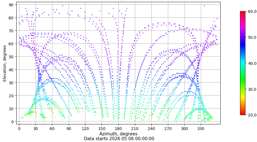
Azimuth-elevation plot for station VIGO. Signal to Noise S1C Data file VIGO00ESP_R_2026126.xtr
