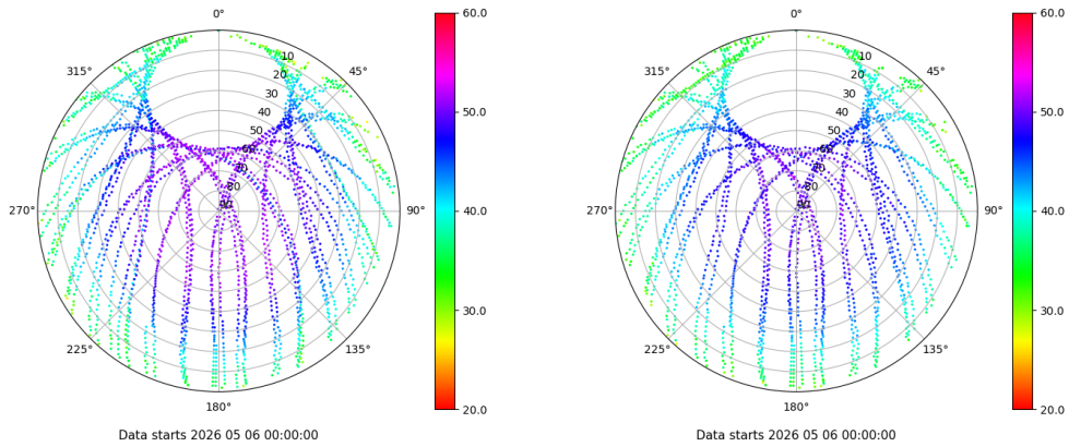
Skyplot for station VIGO. Signal to Noise S1C Data file VIGO00ESP_R_2026126.xtr Skyplot for station VIGO. Signal to Noise S2C Data file VIGO00ESP_R_2026126.xtr
