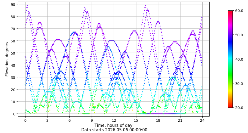
Time-elevation plot for station VIGO. Signal to Noise S1C Data file VIGO00ESP_R_2026126.xtr
