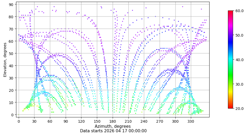
Azimuth-elevation plot for station VIGO. Signal to Noise S1C Data file VIGO00ESP_R_2026107.xtr
