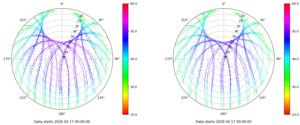
Skyplot for station VIGO. Signal to Noise S1C Data file VIGO00ESP_R_2026107.xtr Skyplot for station VIGO. Signal to Noise S2C Data file VIGO00ESP_R_2026107.xtr
