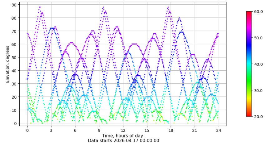
Time-elevation plot for station VIGO. Signal to Noise S1C Data file VIGO00ESP_R_2026107.xtr
