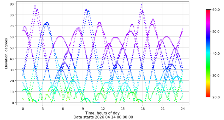
Time-elevation plot for station VIGO. Signal to Noise S1C Data file VIGO00ESP_R_2026104.xtr
