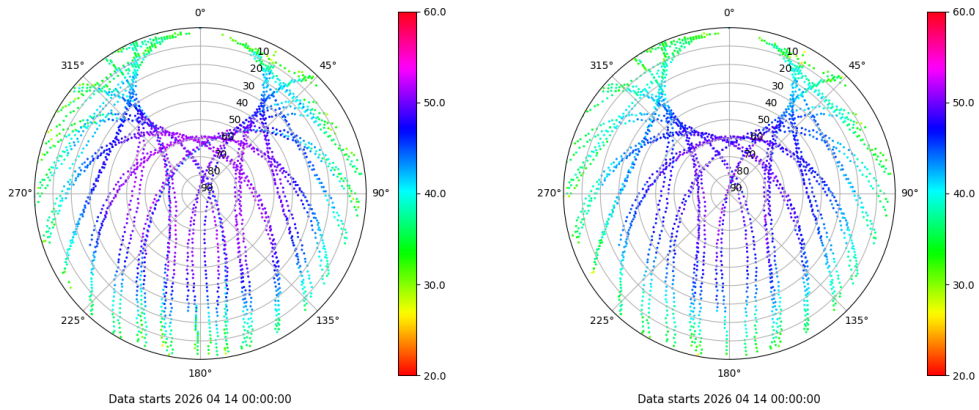
Skyplot for station VIGO. Signal to Noise S1C Data file VIGO00ESP_R_2026104.xtr Skyplot for station VIGO. Signal to Noise S2C Data file VIGO00ESP_R_2026104.xtr
