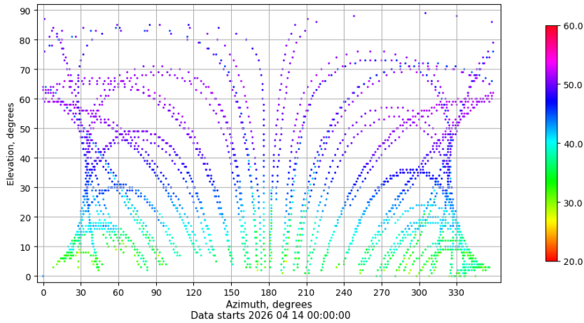
Azimuth-elevation plot for station VIGO. Signal to Noise S1C Data file VIGO00ESP_R_2026104.xtr
