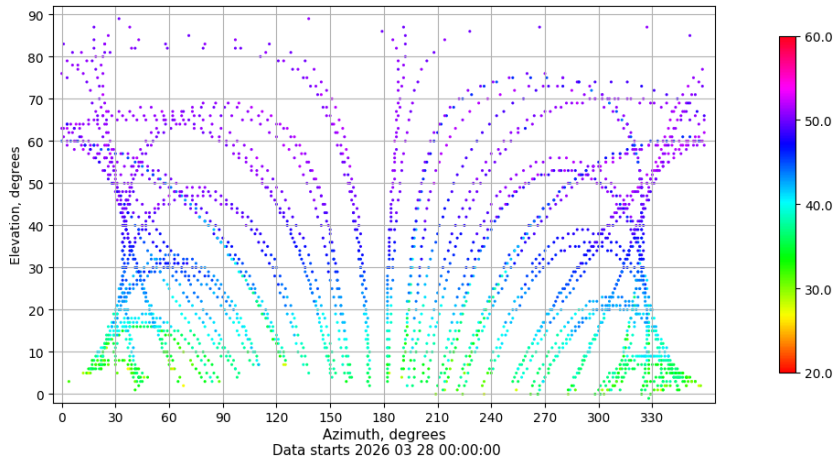
Azimuth-elevation plot for station VIGO. Signal to Noise S1C Data file VIGO00ESP_R_2026087.xtr
