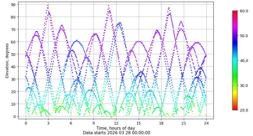
Time-elevation plot for station VIGO. Signal to Noise S1C Data file VIGO00ESP_R_2026087.xtr
