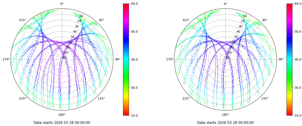
Skyplot for station VIGO. Signal to Noise S1C Data file VIGO00ESP_R_2026087.xtr Skyplot for station VIGO. Signal to Noise S2C Data file VIGO00ESP_R_2026087.xtr
