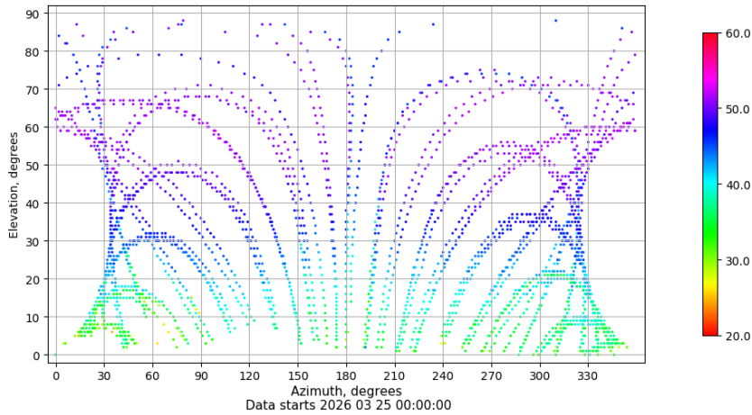
Azimuth-elevation plot for station VIGO. Signal to Noise S1C Data file VIGO00ESP_R_2026084.xtr
