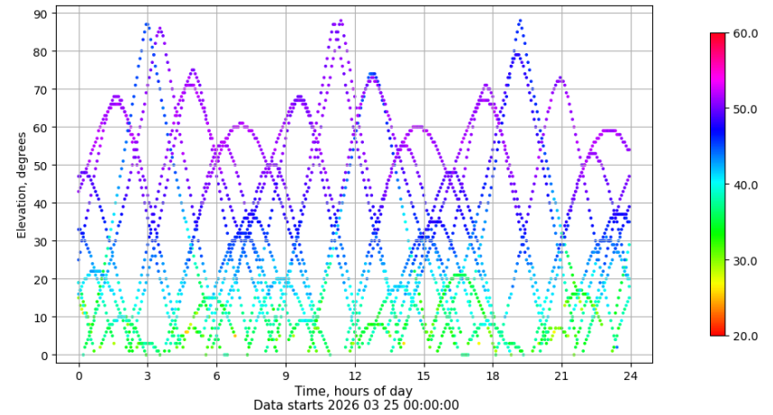
Time-elevation plot for station VIGO. Signal to Noise S1C Data file VIGO00ESP_R_2026084.xtr
