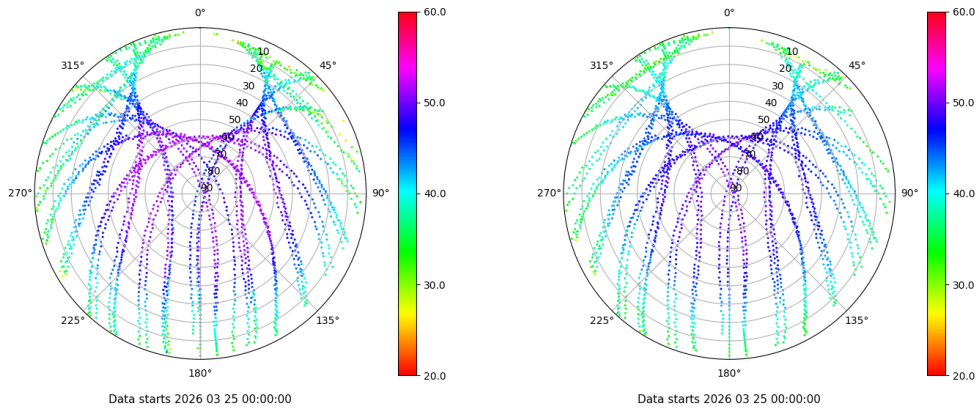
Skyplot for station VIGO. Signal to Noise S1C Data file VIGO00ESP_R_2026084.xtr Skyplot for station VIGO. Signal to Noise S2C Data file VIGO00ESP_R_2026084.xtr
